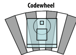
Placement orientation of the encoder's emitter and detector on the codewheel
