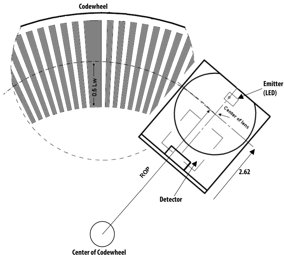
Placement orientation of the encoder's emitter and detector on the codewheel
