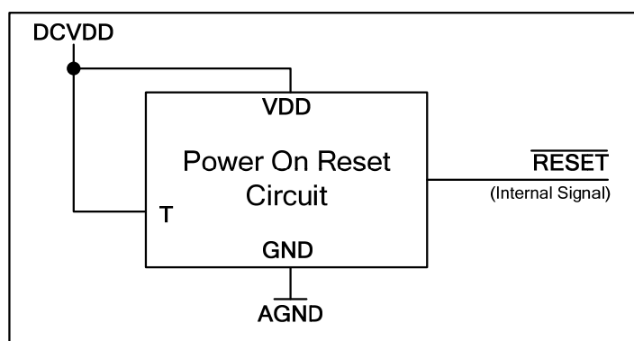
Figure 2 Internal Power on Reset Circuit Schematic
