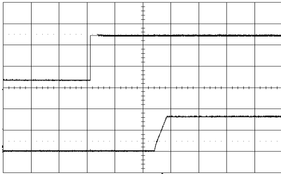
Start-up enabled by connecting V_I at: T_{P1} = +25^\circ\text{C} , V_I = 12\text{ V} , V_O = 3.3\text{ V} C_O = 470\ \mu\text{F}/10\ \text{m}\Omega , I_O = 12\text{ A} Top trace: Input voltage (5 V/div.). Bottom trace: Output voltage (2 V/div.). Time scale: (20 ms/div.).
