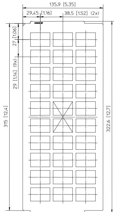
X = Vacuum pickup area.
