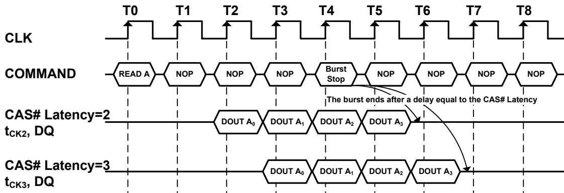
Figure 17. Termination of a Burst Read Operation (Burst Length > 4, CAS# Latency = 2, 3)
