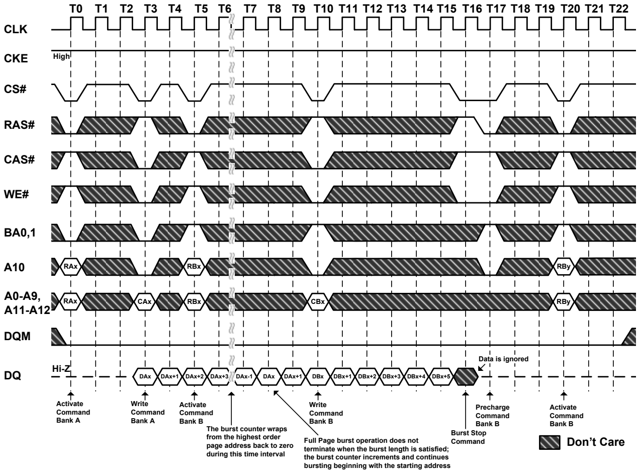
Figure 38. Full Page Write Cycle (Burst Length=Full Page)
