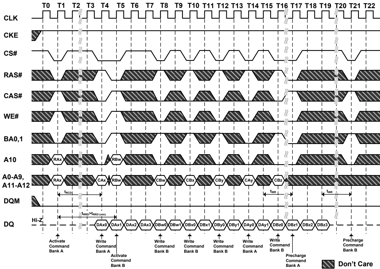
Figure 34. Interleaved Column Write Cycle (Burst Length=4)
