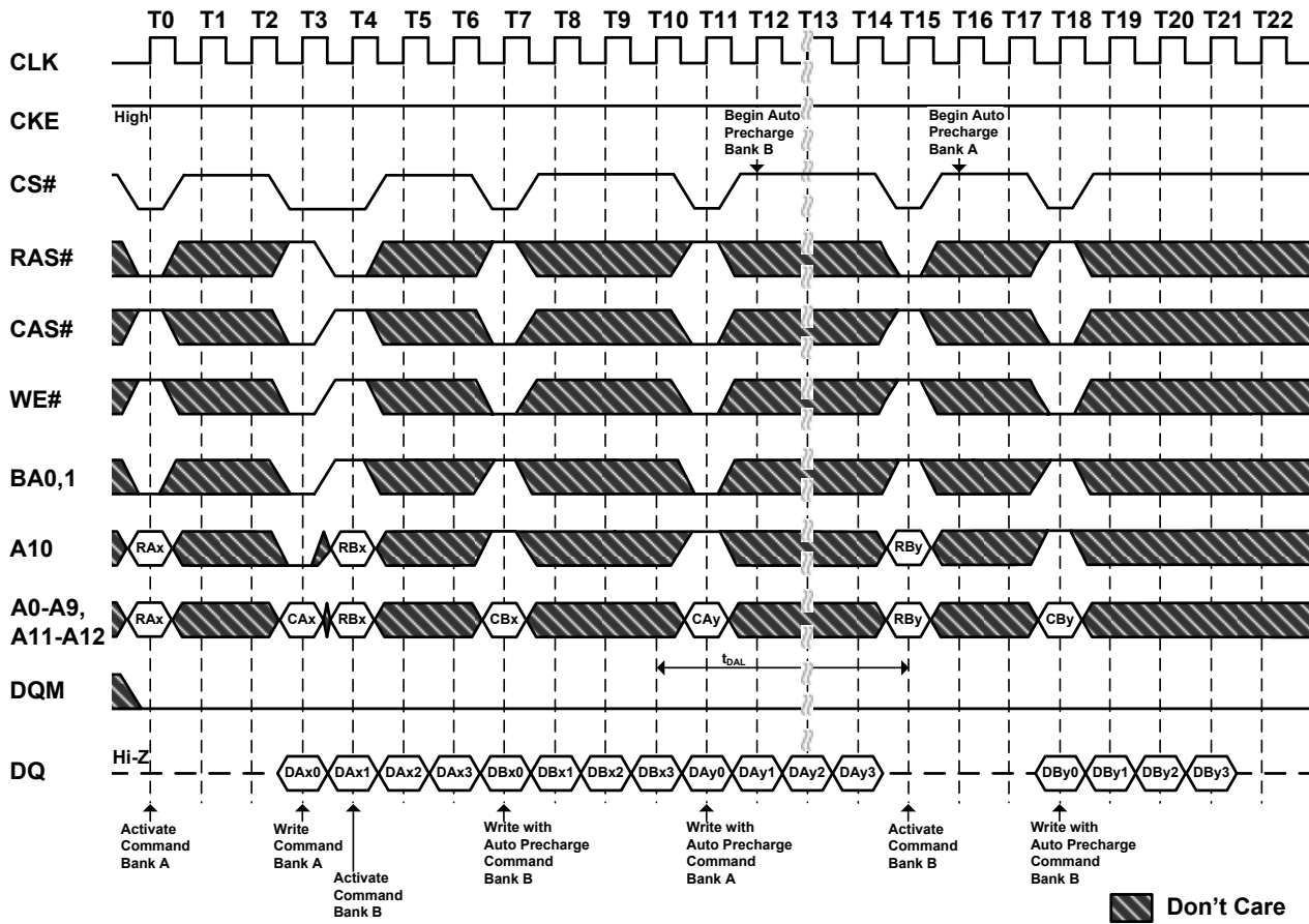
Figure 36. Auto Precharge after Write Burst (Burst Length=4)
