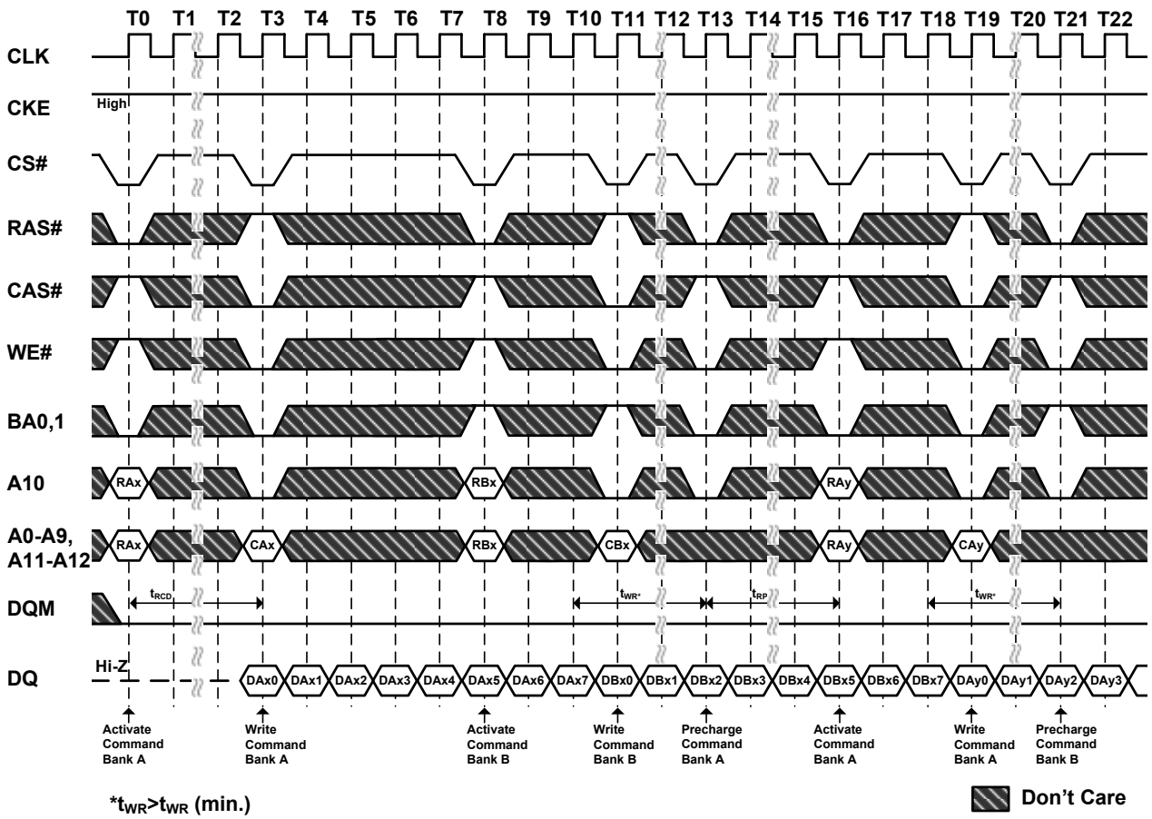
Figure 31. Random Row Write (Interleaving Banks) (Burst Length=8)
