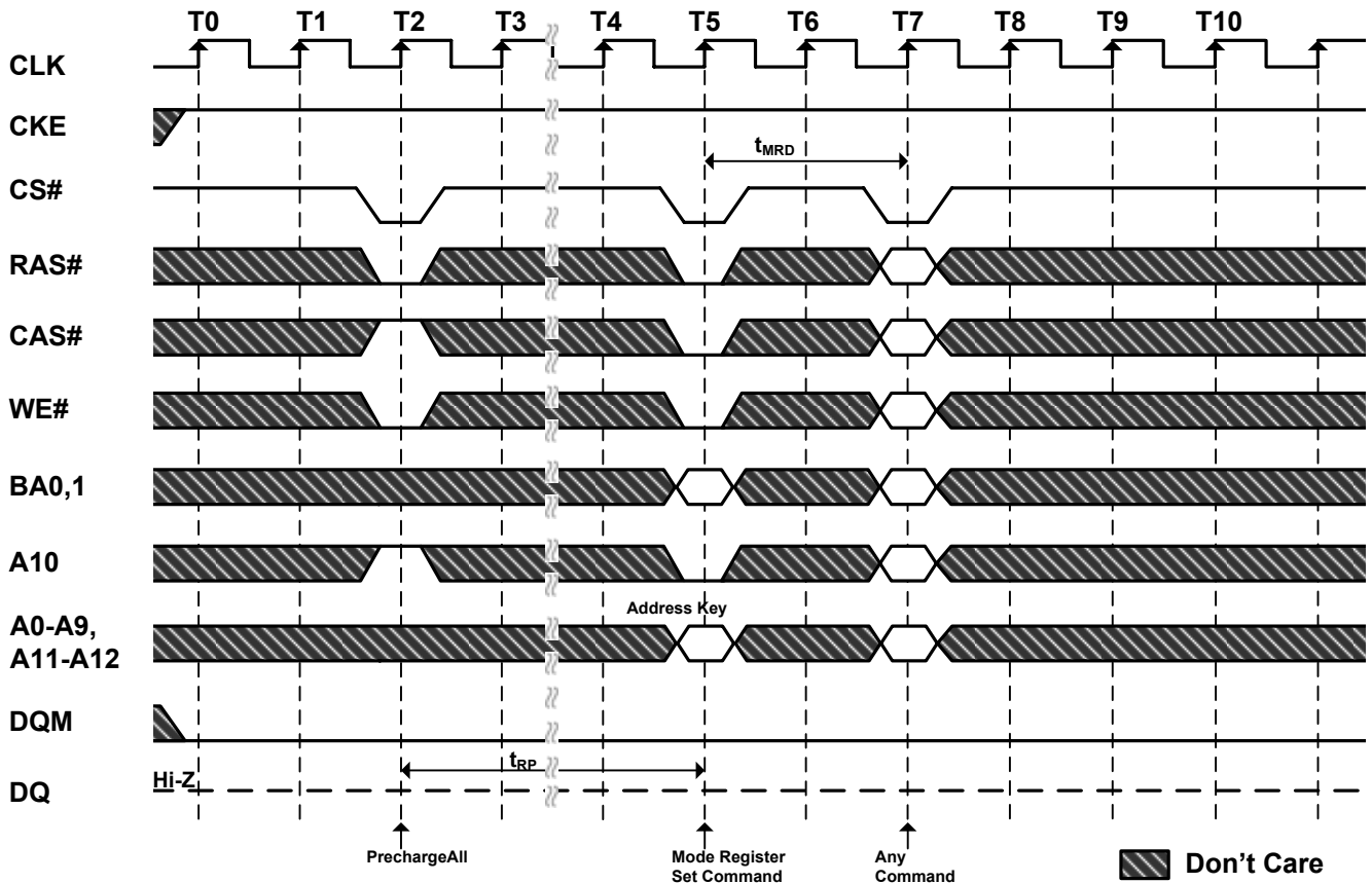
Figure 16. Mode Register Set Cycle
