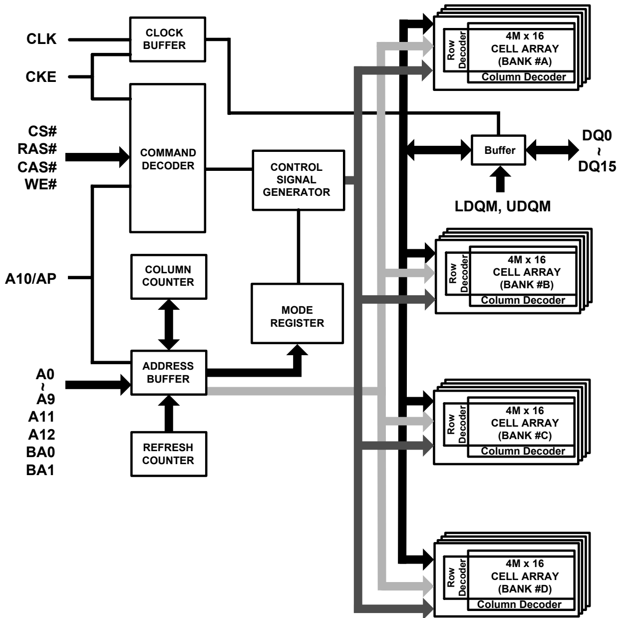
Figure 3. Block Diagram
