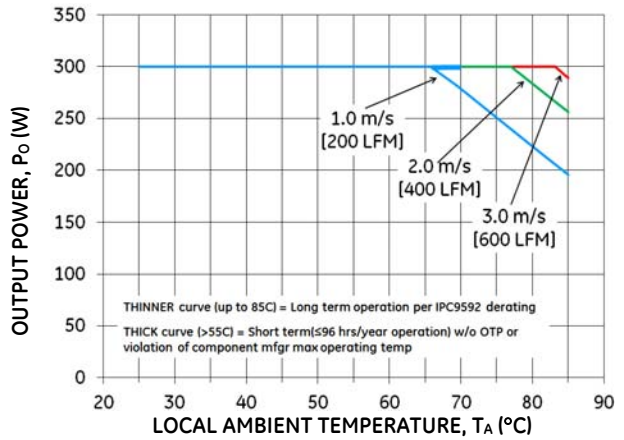
Figure 18. Output Power Derating for the EBVE031A0S9R6-H Base Plate Option in the Longitudinal Orientation; Airflow Direction from Vout or Vin edge; Vin = 38 to 42V.
