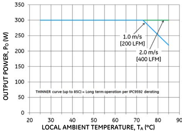
Figure 16. Output Power Derating for the EBVE031A0S9R6-H Base Plate Option in the Transverse Orientation; Airflow Direction from Vin(-) to Vin(+); Vin = 50V.
