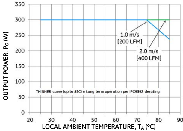
Figure 15. Output Power Derating for the EBVE031A0S9R6-H Base Plate Option in the Transverse Orientation; Airflow Direction from Vin(-) to Vin(+); Vin = 38 to 42V.
