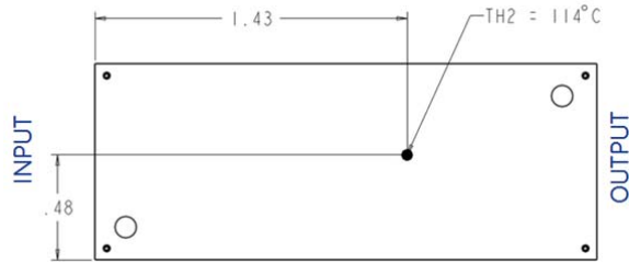
Figure 13. Location of the thermal reference temperature Tref.
