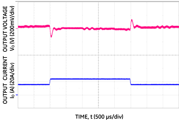
Figure 4. Typical Transient Response to 1A/ \mu s Step Change in Load from 50% to 75% to 50% of Full Load, C_o = 1200\mu F and 50 V dc Input.
