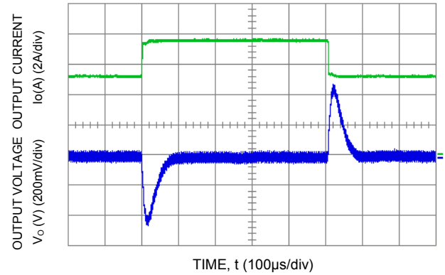
Figure 4. Transient Response to 1.0A/ \mu s Dynamic Load Change from 50% to 75% to 50% of full load ( V_{IN} = V_{IN,NOM} ).
