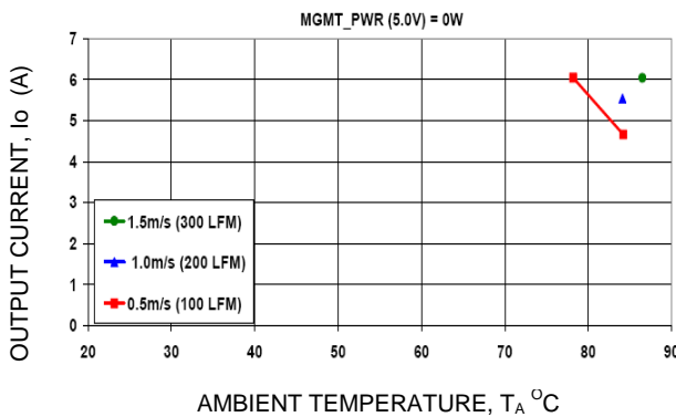
Figure 14-1. PIM300A Derating Output Current versus Local Ambient Temperature and Airflow (Vin = -48Vdc; MGMT_PWR, 5.0V=0W)
