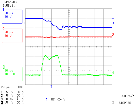
Figure 2. Inrush Current
