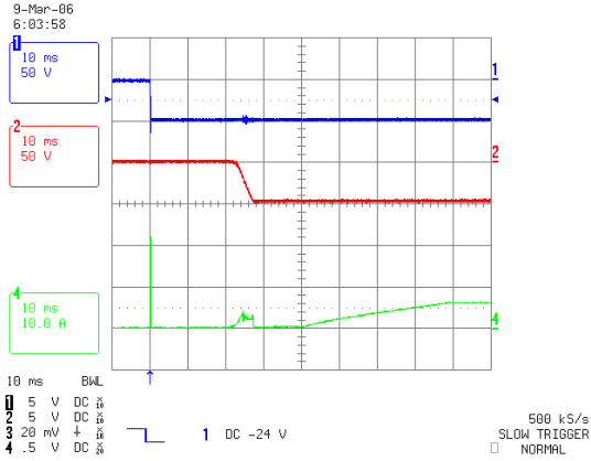
Figure 1. Inrush Current
