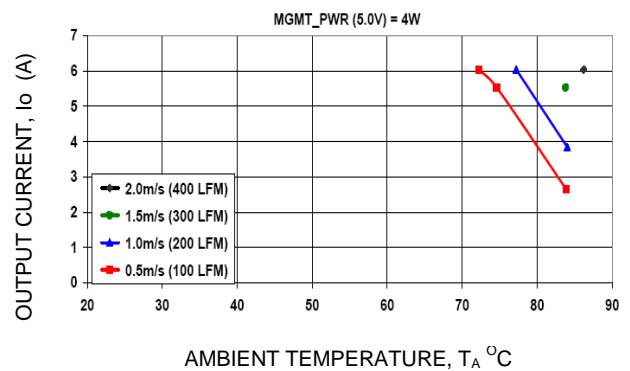
Figure 14-2. PIM300A Derating Output Current versus Local Ambient Temperature and Airflow (Vin = -48Vdc; MGMT_PWR, 5.0V=4W)
