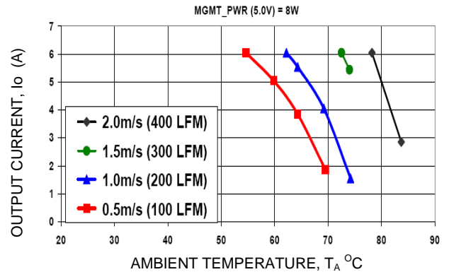
Figure 14-4. PIM300A Derating Output Current versus Local Ambient Temperature and Airflow (Vin = -48Vdc; MGMT_PWR, 5.0V=8W)
