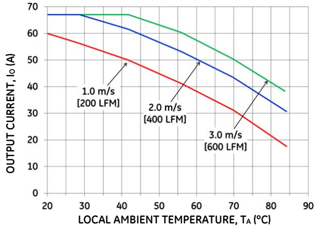
Figure 17. Output Current Derating for the Base Plate QBVE067A0Bxx-H in the Transverse Orientation; Airflow Direction from Vin(-) to Vin(+); Vin = 50V.
