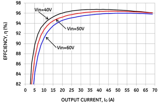
Figure 2. Typical Converter Efficiency vs. Output Power.
