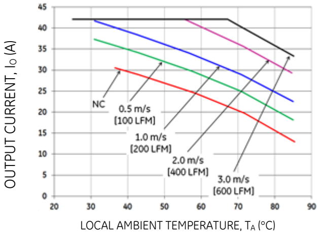
Figure 18. Output Current Derating for the Base plate QSVW042A0B in the Transverse Orientation; Airflow Direction from Vin(-) to Vin(+); Vin = 48V.
