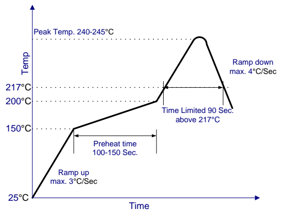
Figure 20. Recommended linear reflow profile using Sn/Ag/Cu solder.
