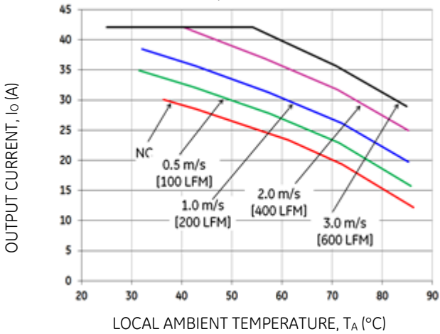
Figure 19. Output Current Derating for the Base plate QSVW042A0B-H in the Longitudinal Orientation; Airflow Direction from Vin(-) to Vin(+); Vin = 48V.
