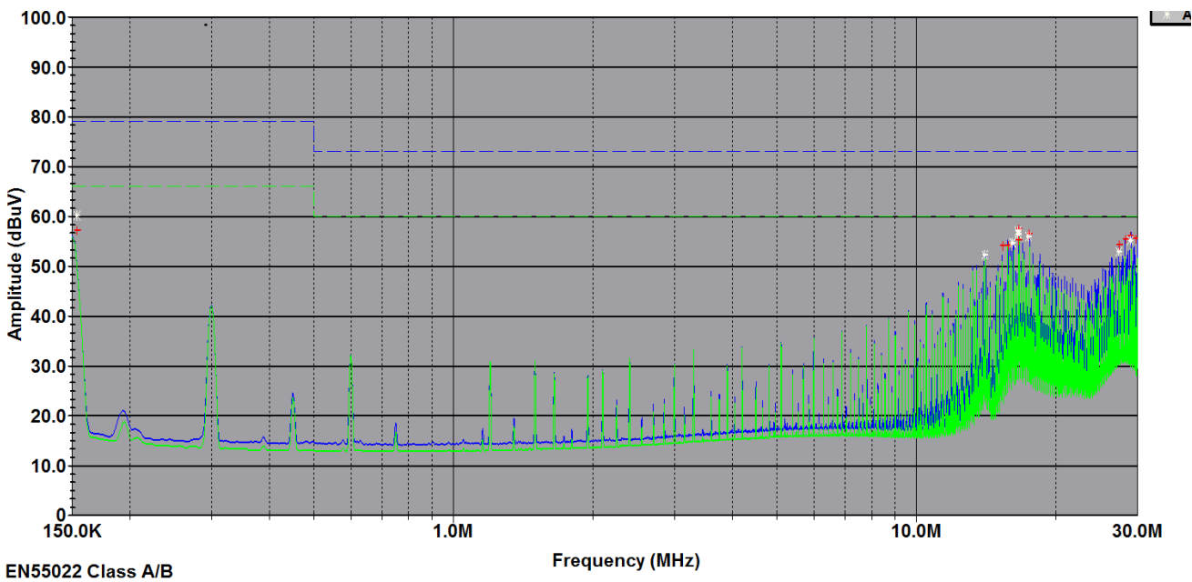
Figure 21. EMC Consideration
