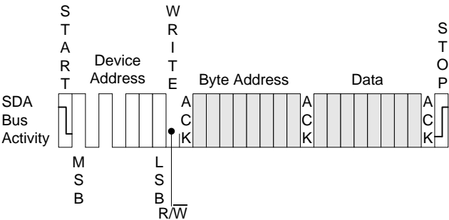
Figure 5-6. Byte Write
