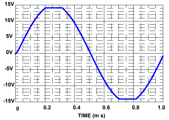
FIGURE 61. SIMULATED OUTPUT VOLTAGE SWING ±15V
