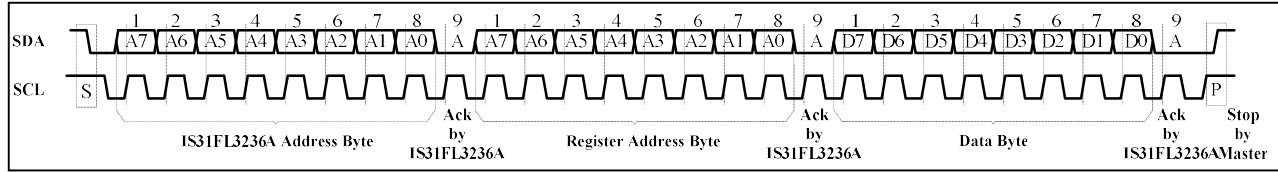
Figure 4 Writing to IS31FL3236A(Typical)
