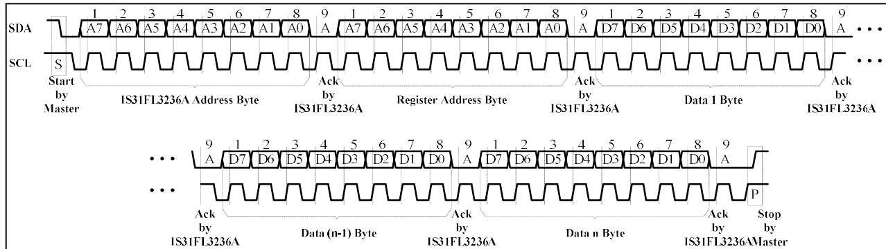
Figure 5 Writing to IS31FL3236A(Automatic address increment)
