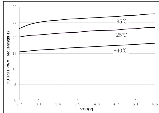
Figure 8 VCC vs. OUTPUT PWM Frequency
