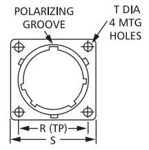
RECEPTACLE ASSEMBLY
