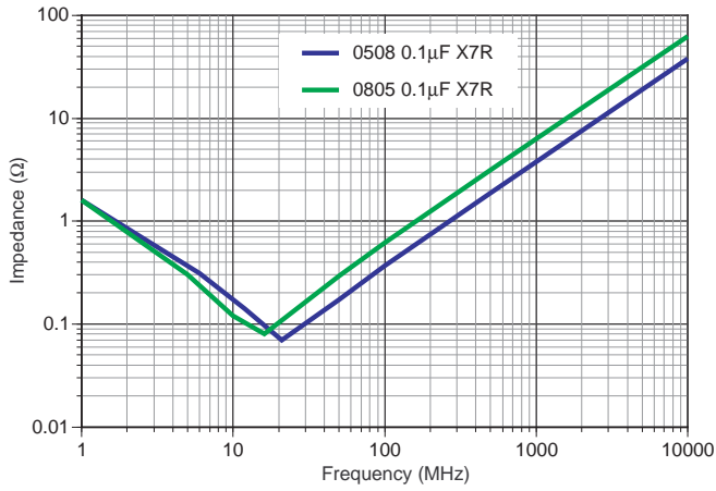
IMPEDANCE 0508 vs. 0805
