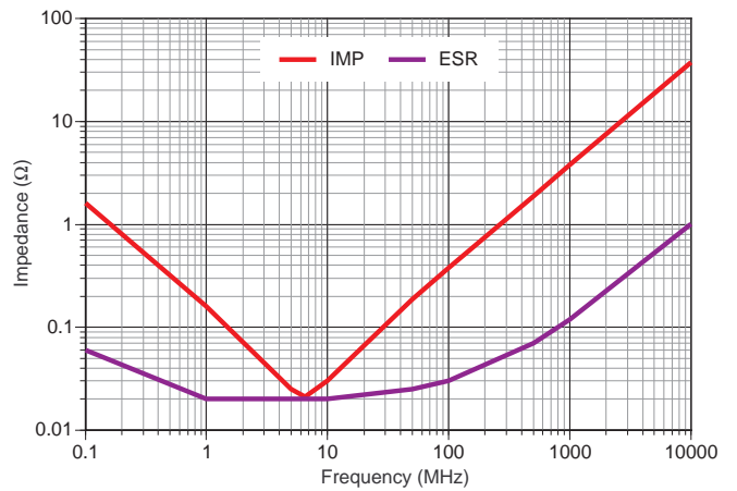
IMPEDANCE AND ESR 0612 0.1μF X7R
