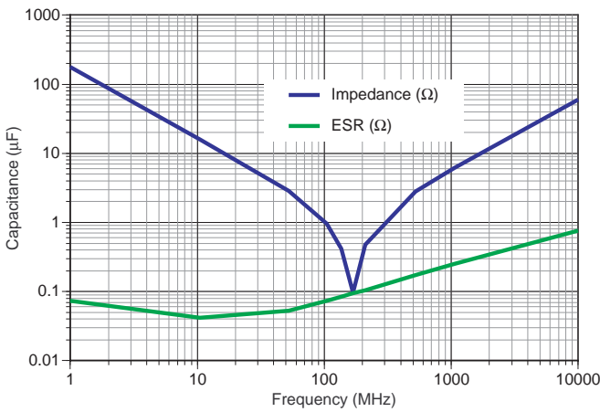
IMPEDANCE AND ESR 0612 0.1μF X7R
