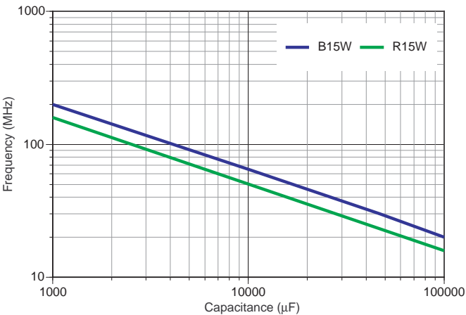
SERIES RESONANT FREQUENCY 0508 vs. 0805
