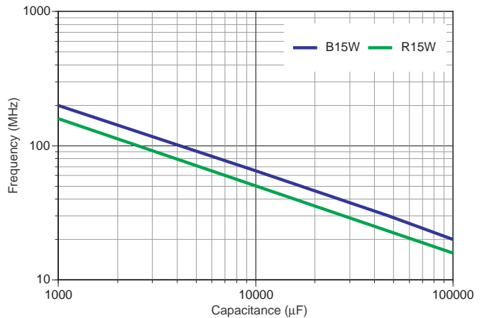
0508 X7R SERIES RESONANT FREQUENCY
