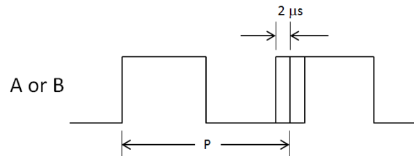
Figure 13: ABZ Jitter
