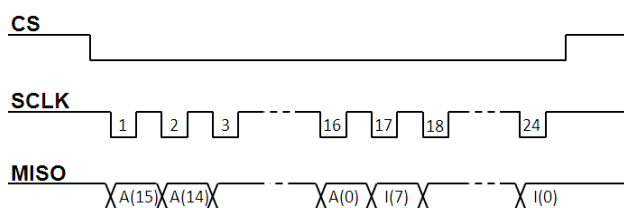
Figure 11: Timing Diagram for SPI Angle + Index Readout
