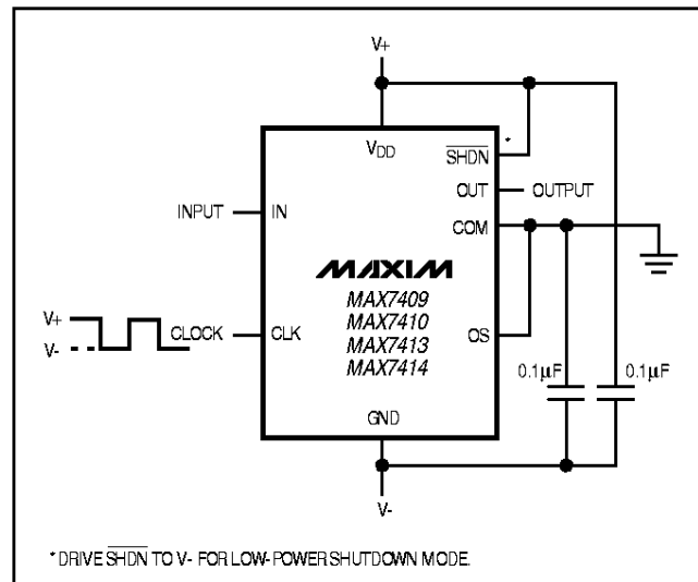
Figure 4. Dual-Supply Operation
