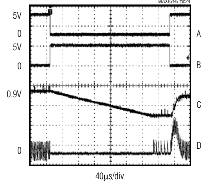
A. \overline{\text{DPRSTP}} , 5V/div B. DPRSLPVR, 5V/div C. V_{OUT} , 200mV/div D. INDUCTOR CURRENT, 10A/div I_{OUT} = 1\text{A}
