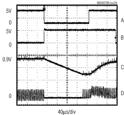
A. \overline{\text{DPRSTP}} , 5V/div B. DPRSLPVR, 5V/div C. V_{OUT} , 200mV/div D. INDUCTOR CURRENT, 10A/div I_{OUT} = 2\text{A}
