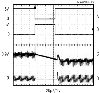
A. \overline{\text{DPRSTP}} , 5V/div B. DPRSLPVR, 5V/div C. V_{OUT} , 20mV/div D. INDUCTOR CURRENT, 10A/div I_{OUT} = 0.3\text{A}
