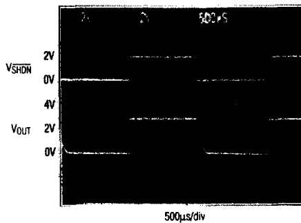
MAX8866 SHUTDOWN (50mA LOAD)
