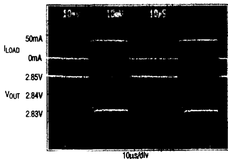
LOAD-TRANSIENT RESPONSE
