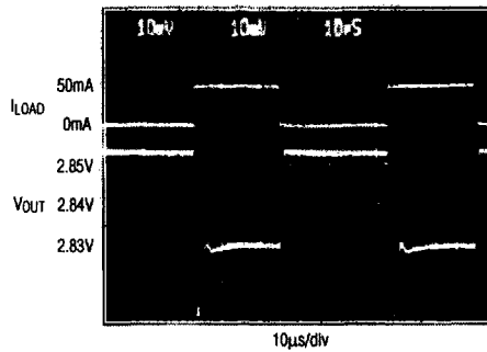
LOAD-TRANSIENT RESPONSE
