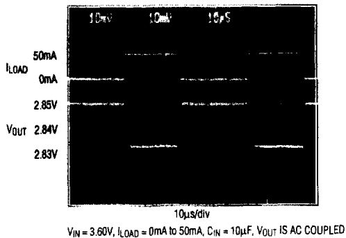
LOAD-TRANSIENT RESPONSE
