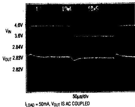
LINE-TRANSIENT RESPONSE
