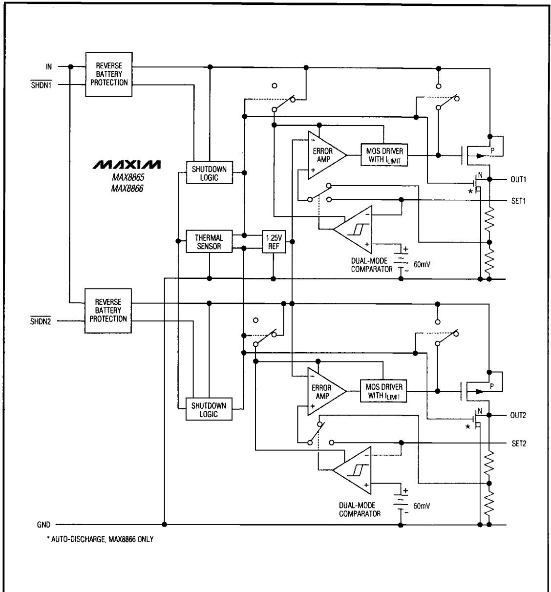
Figure 1. Functional Diagram
