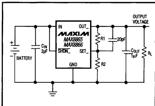
Figure 2. Adjustable Output Using External Feedback Resistors
