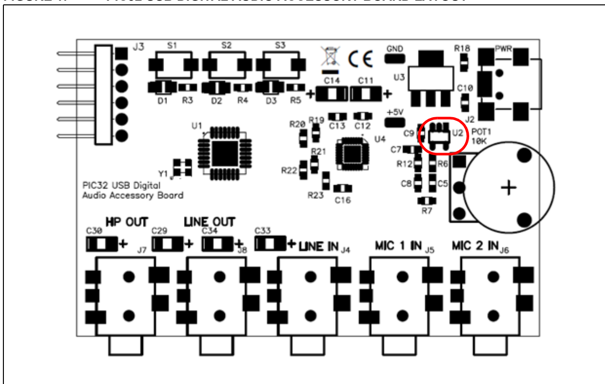
FIGURE 1: PIC32 USB DIGITAL AUDIO ACCESSORY BOARD LAYOUT
