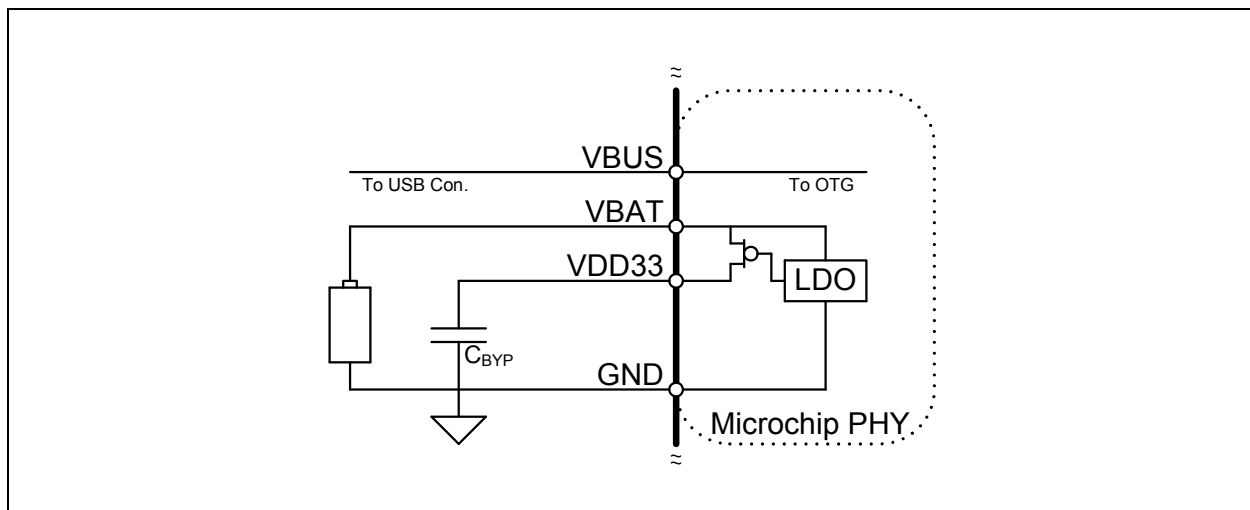
FIGURE 5-3: POWERING THE USB3318 FROM A BATTERY
