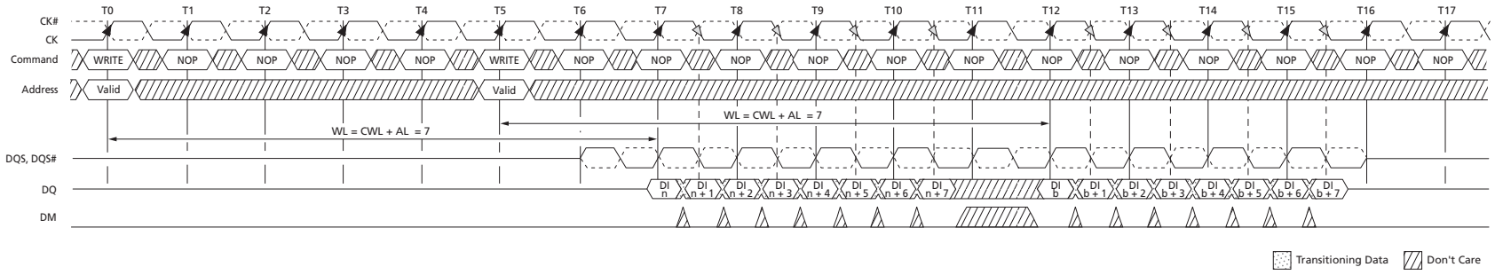
Figure 89: Nonconsecutive WRITE to WRITE
