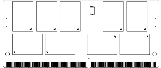
Figure 1: 260-Pin SODIMM (MO-310 R/C H)
