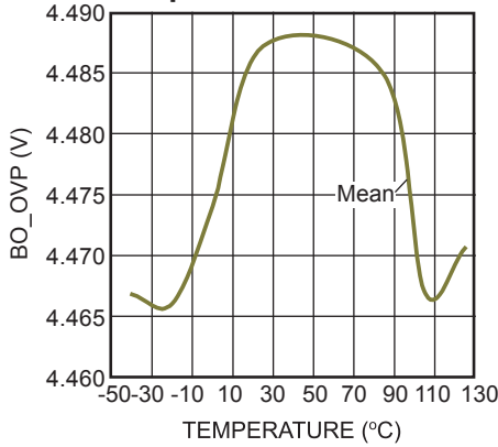
BO_OVP vs. Temperature
