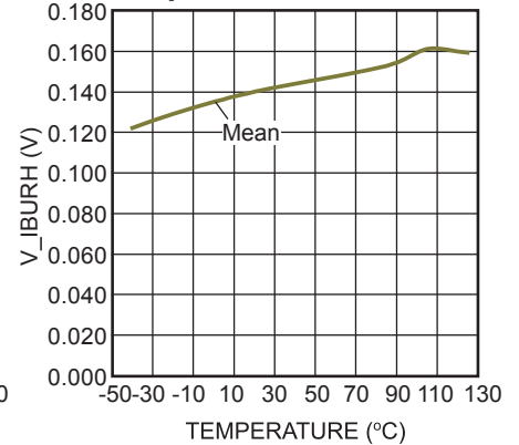
V_IBURH vs. Temperature
