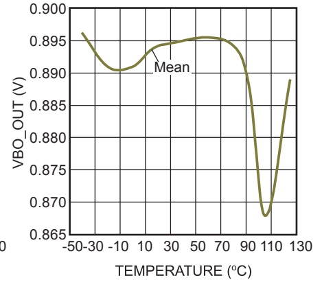
VBO_OUT vs. Temperature
