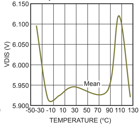
VDIS vs. Temperature
