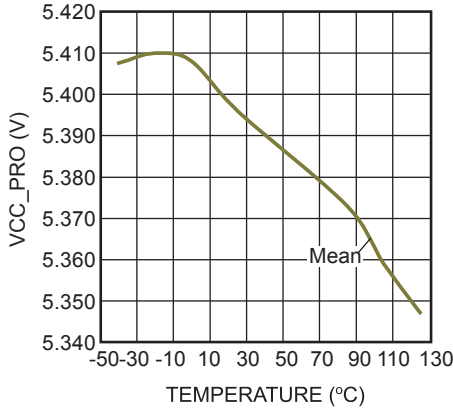
VCC_PRO vs. Temperature
