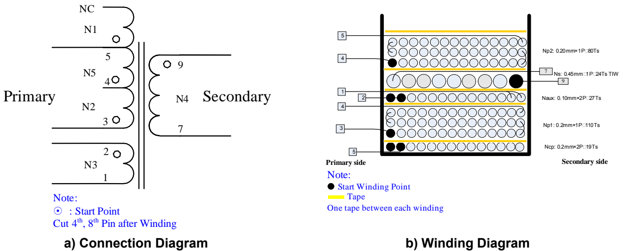
Figure 15: Transformer Structure
