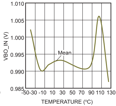
VBO_IN vs. Temperature
