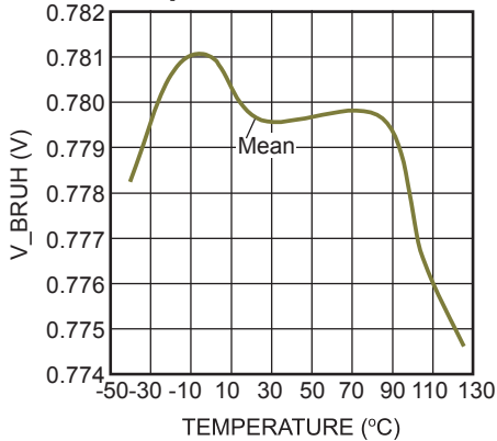
V_BRUH vs. Temperature
