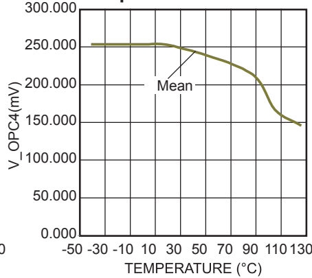
V_OPC4 vs. Temperature Chart
