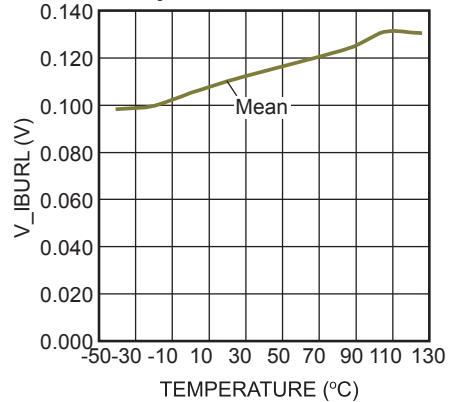
V_IBURL vs. Temperature
