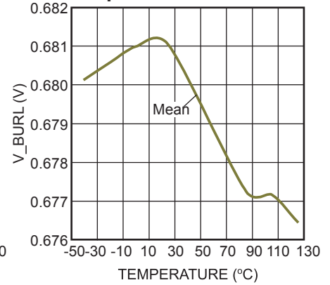
V_BURL vs. Temperature
