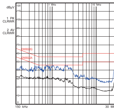
Conducted EMI, L
