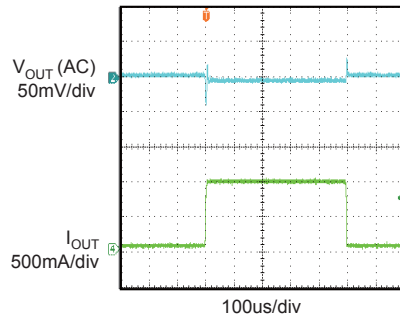
Load Transient
