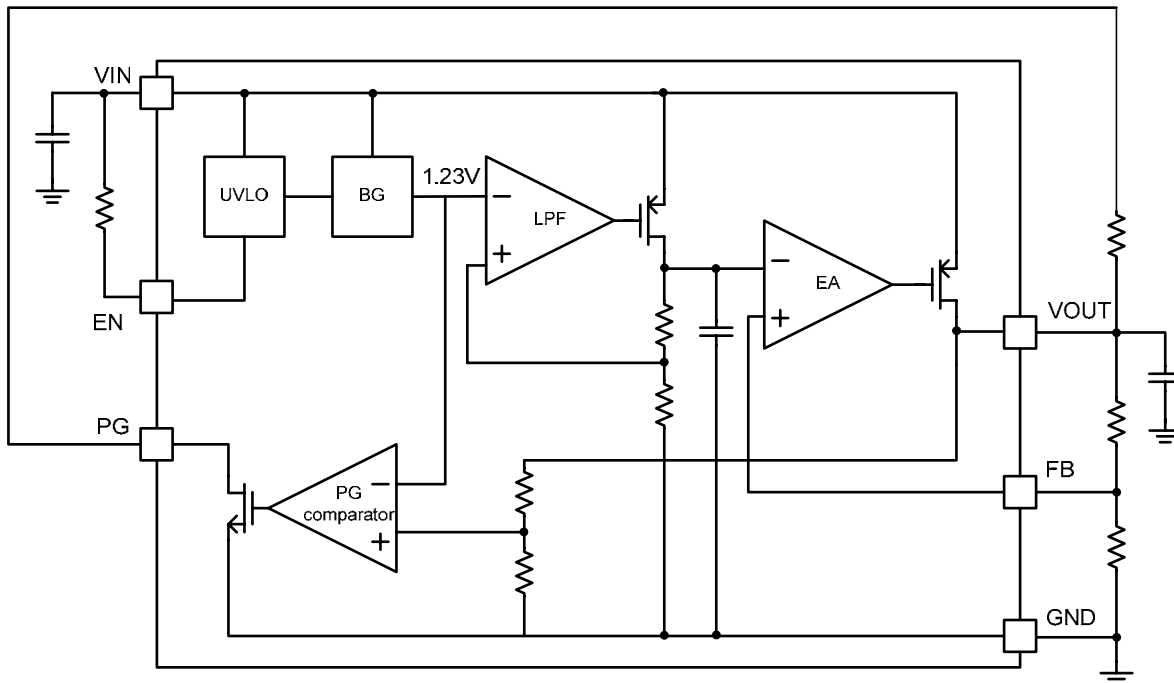
Figure 1—Block Diagram of Super Low Dropout Regulation
