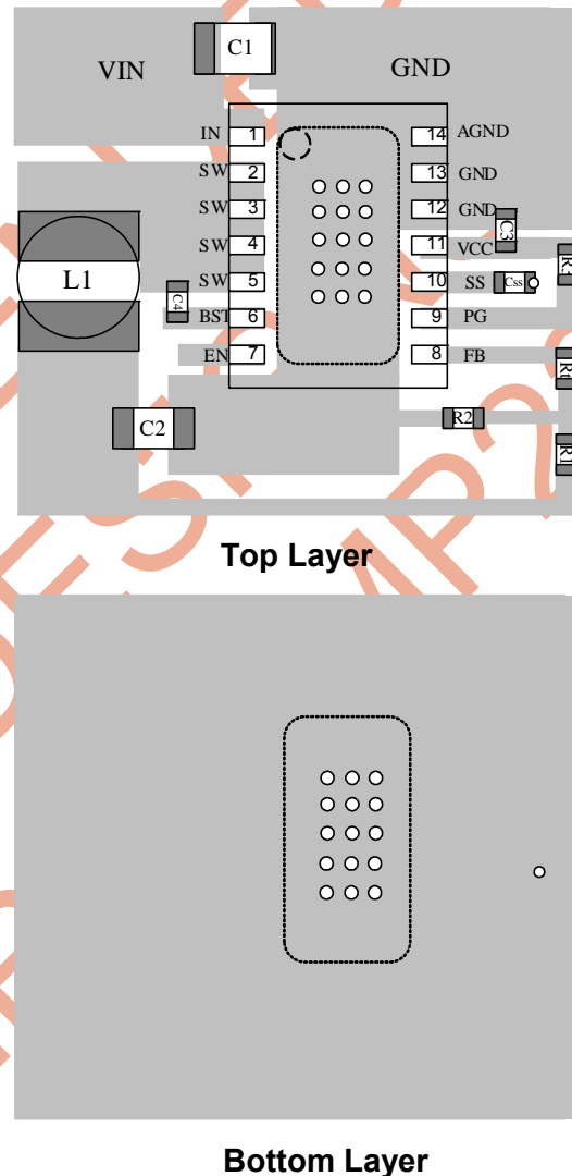
Figure 7—PCB Layout
