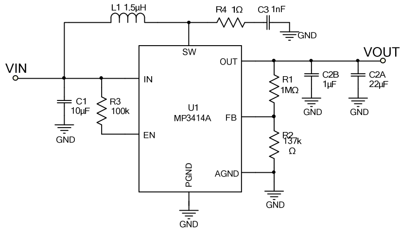
Figure 3: Typical Boost Application Circuit, V_{IN} = 2.8V to 4.2V , V_{OUT} = 5V , I_{OUT} = 0A-1A
