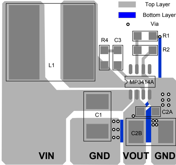
Figure 2: Recommended PCB Layout
