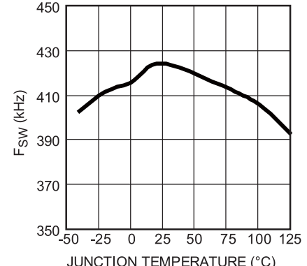
F_{SW} vs. Junction Temperature V_{IN}=12V
