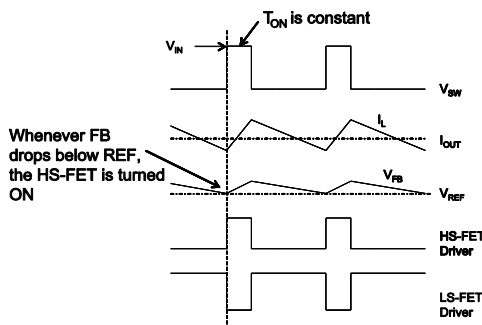
Figure 2: PWM Operation
