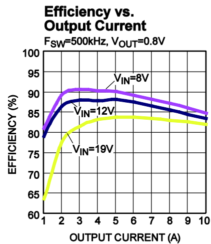
Figure 21 — Efficiency Curve
