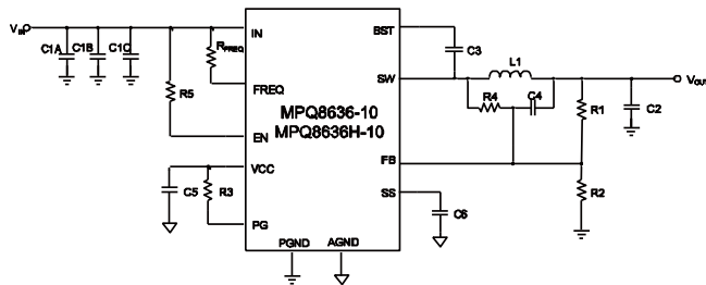
Figure 52—Schematic for PCB Layout Guide
