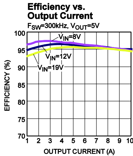
Figure 47 — Efficiency Curve MPQ8636-10, MPQ8636H-10, V_{OUT}=5V , I_{OUT}=1A-10A , f_{SW}=300kHz
