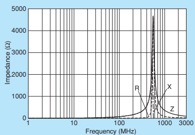
BLM15BA750SN1
