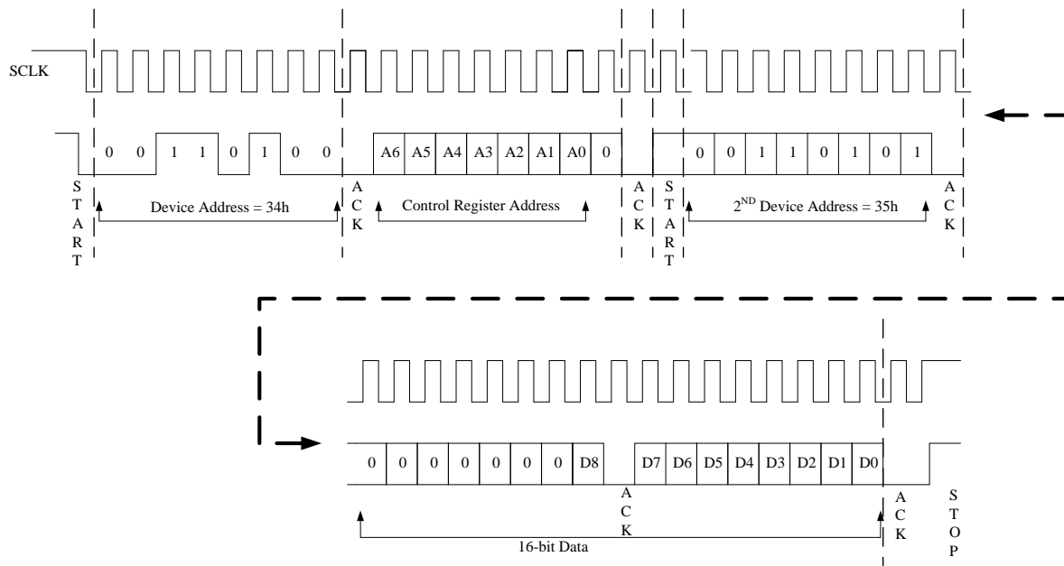
Figure 11: Read Sequence
