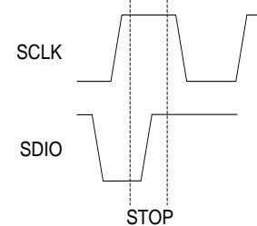
Figure 8: Valid STOP Condition
