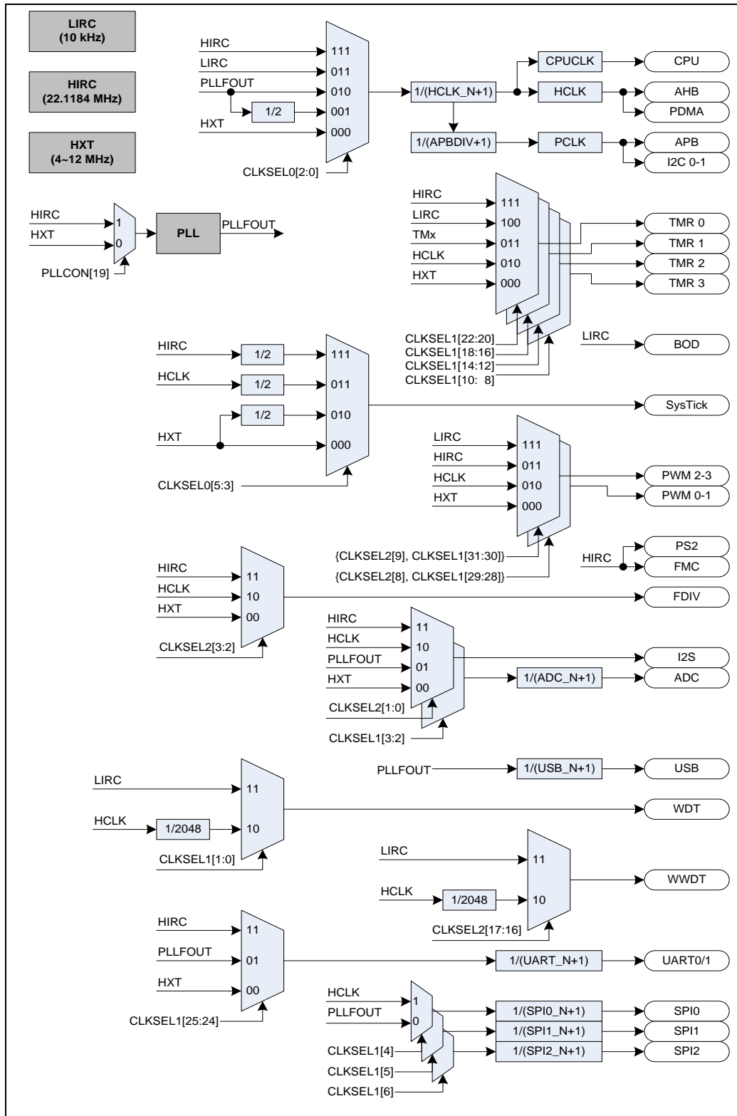
Figure 5-2 Clock Generator Global View Diagram
