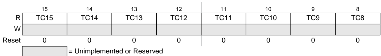
Figure 7-59. Timer Input Capture Holding Register 1 High (TC1H)
