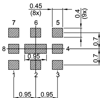
Figure 2: Drawing of package with package height A = 0.5 mm (max.). See Sec. Package information (p. 23).
