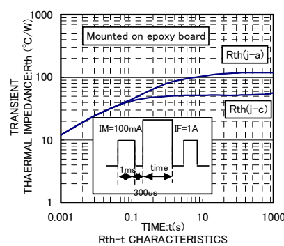
Rth-t CHARACTERISTICS
