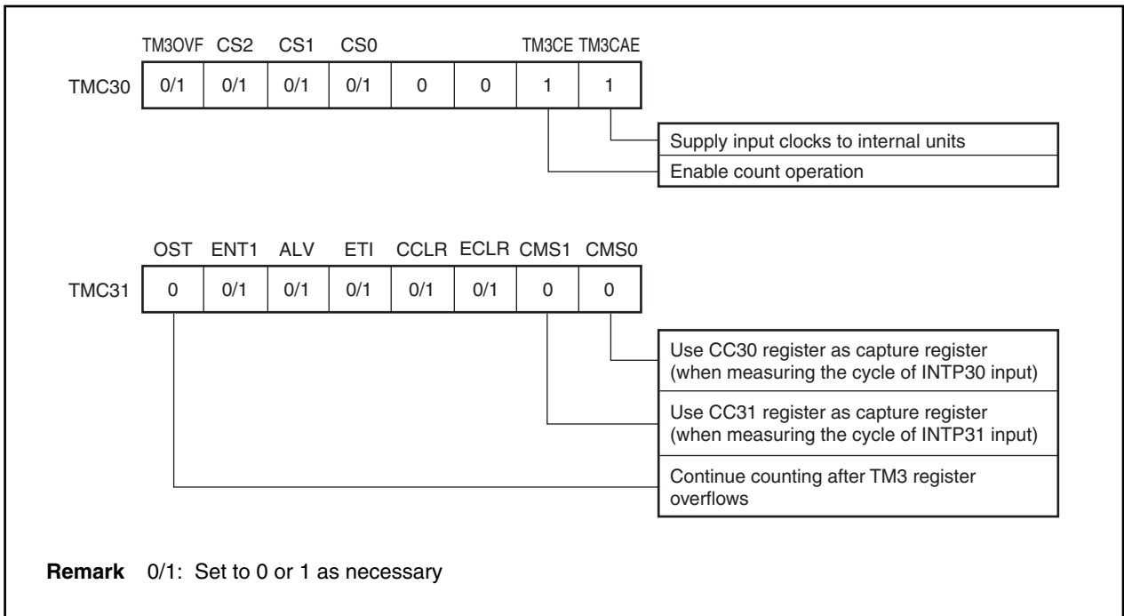
Figure 9-101. Contents of Register Settings When Timer 3 Is Used for Cycle Measurement
