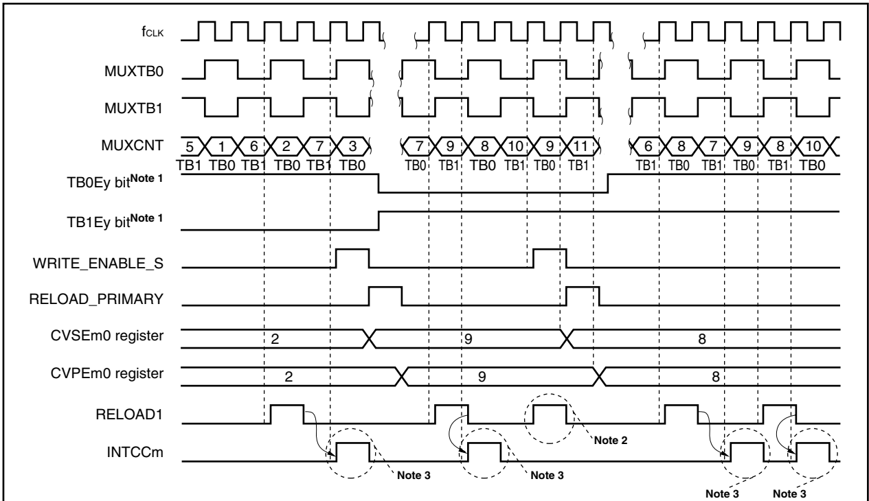
Figure 9-78. Compare Operation: Buffer-Less Mode (When CMSEx0 Register's CCSEy Bit = 1, LNKEY Bit = Arbitrary, BFEEy Bit = 0)
