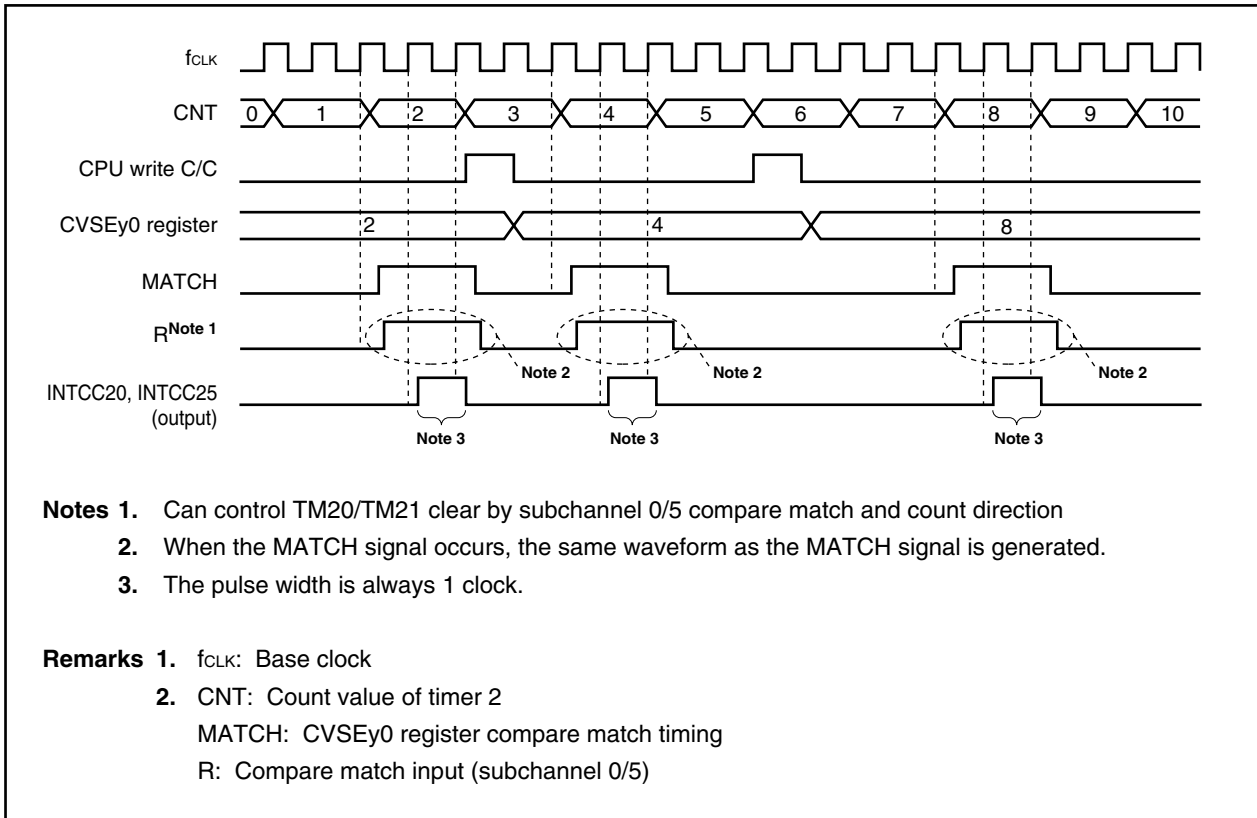
Figure 9-81. Compare Operation: Timing of Compare Match and Write Operation to Register (When CMSE050 Register's CCSEy Bit = 1, EEVEy Bit = Arbitrary, and CSCE0 Register's SEVEy Bit = Arbitrary)
