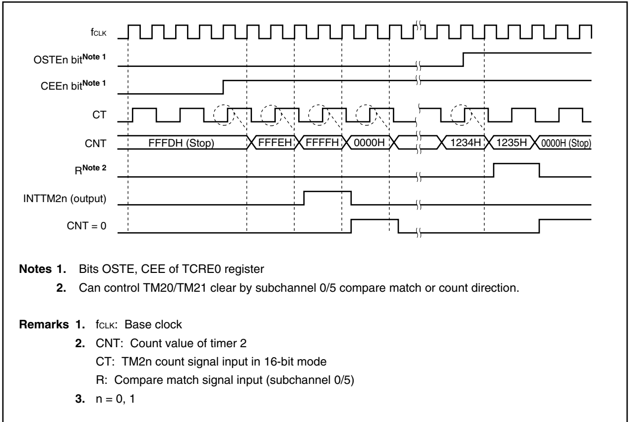
Figure 9-68. Timer 2 Count Up Timing (When TCRE0 Register's UDSEn1, UDSEn0 Bits = 00B, ECEEen Bit = 0, ECREn Bit = 0, CLREn Bit = 0, CASE1 Bit = 0)
