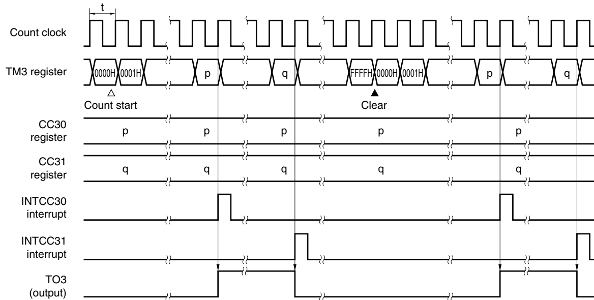
Figure 9-100. PWM Output Operation Timing Example
