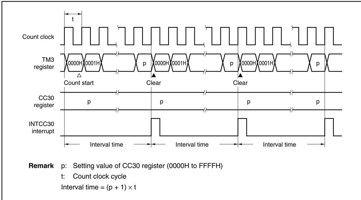
Figure 9-98. Interval Timer Operation Timing Example
