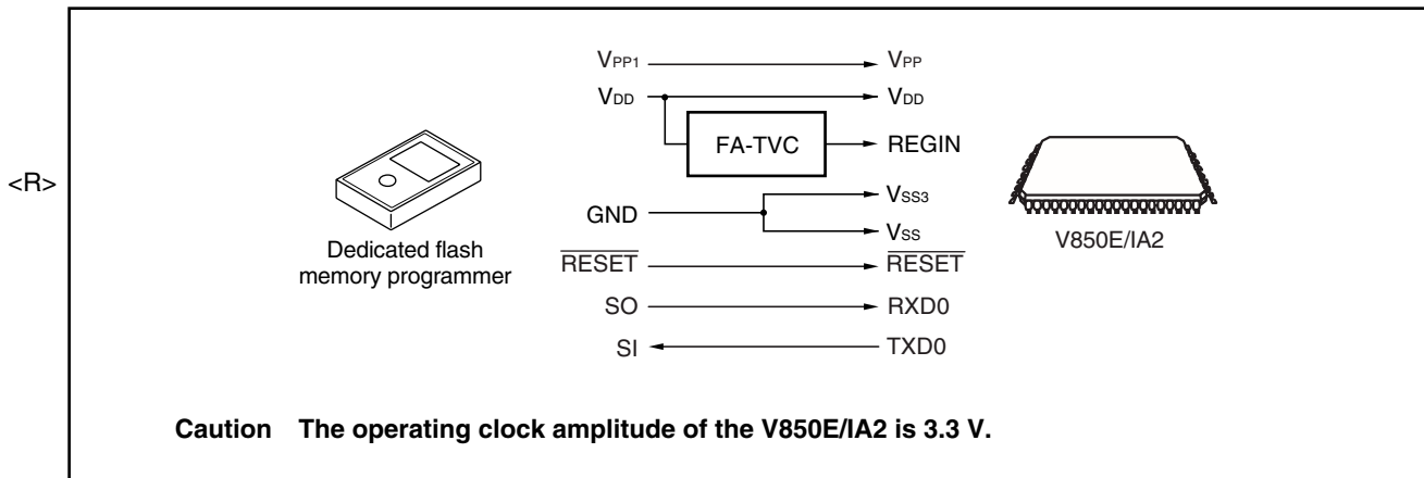
Figure 15-2. Communication with Dedicated Flash Memory Programmer (UART0)
