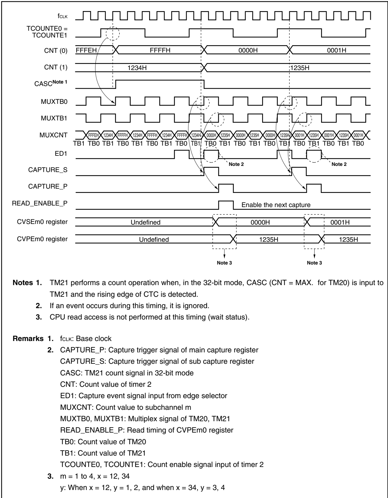
Figure 9-76. Capture Operation: 32-Bit Cascade Operation Mode (When CMSEx Register's TByE1 Bit = 1, TByE0 Bit = 1, CCSEy Bit = 0, LNKEy Bit = 0, BFEEy Bit = Arbitrary, EEVEy Bit = 1, and CSCE0 Register's SEVEy Bit = 0)
