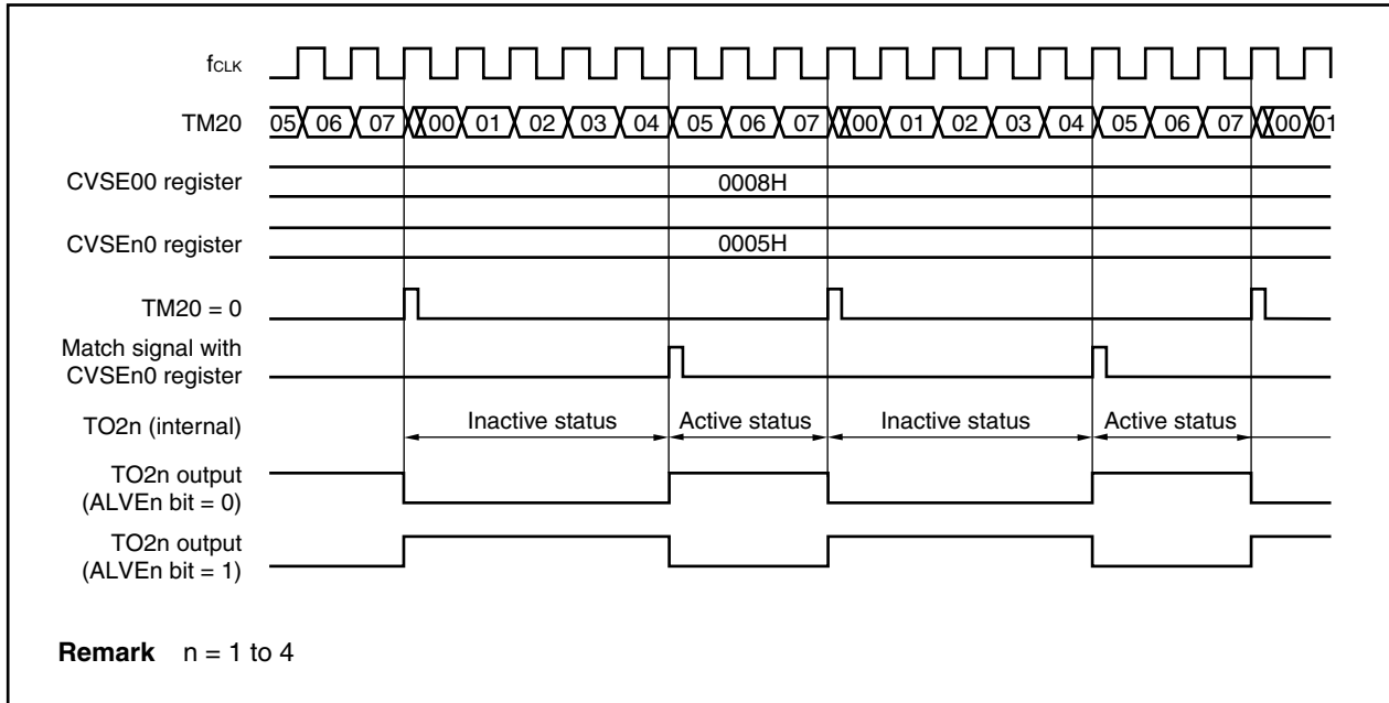
Figure 9-86. During Normal Output Operation
