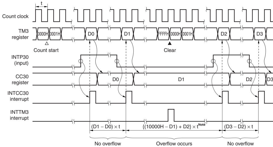
Figure 9-102. Cycle Measurement Operation Timing Example
