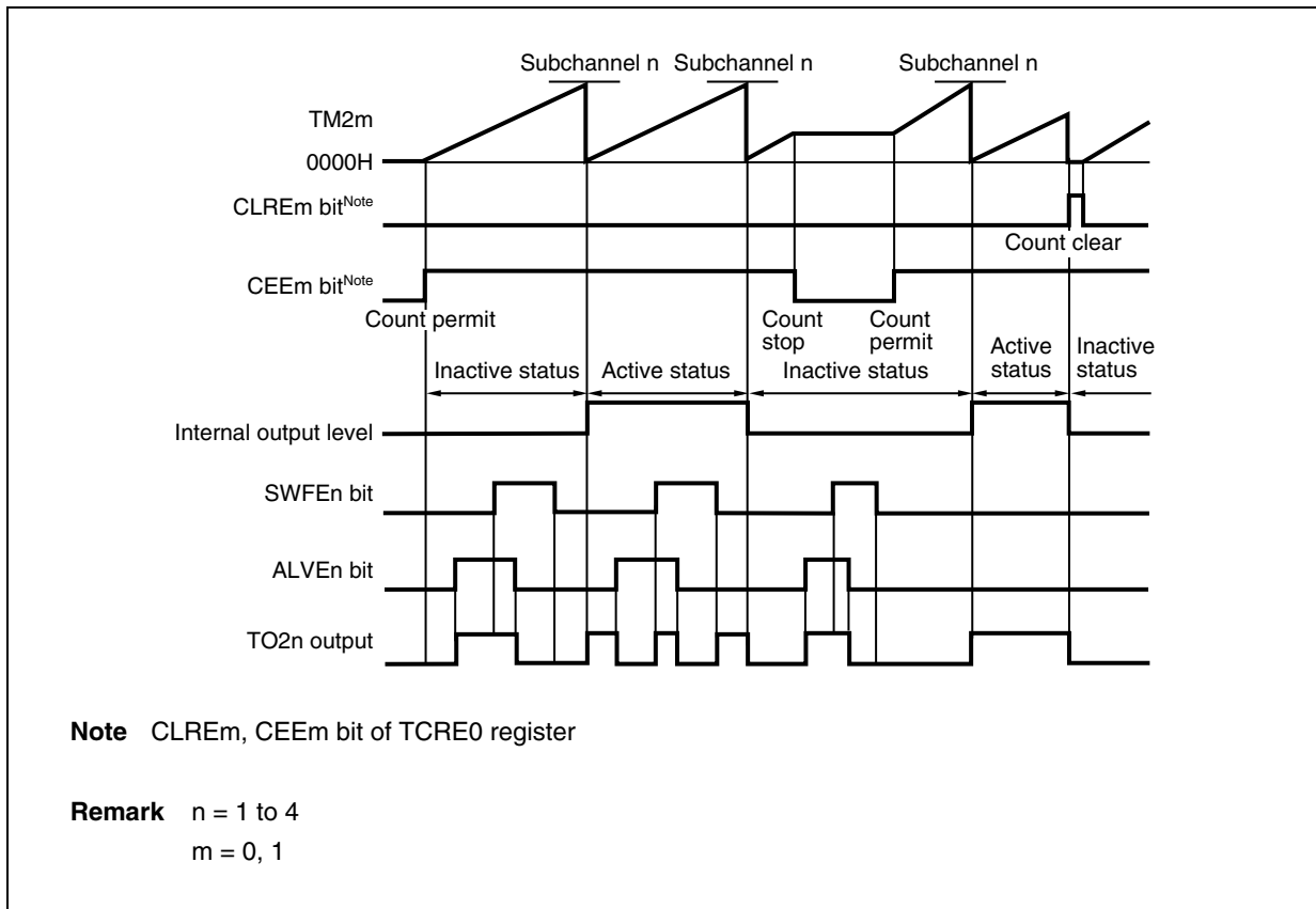
Figure 9-66. Example of Timer Output Timing in Toggle Mode 0
