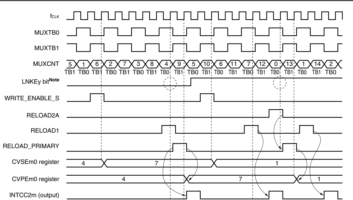
Figure 9-79. Compare Operation: Mode with Buffer (When Operation Is Delayed Through Setting of LNKEY Bit of CMSEx0 Register, CMSEx0 Register's CCSEy Bit = 1, BFEEy Bit = 1)
