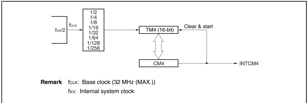
Figure 9-103. Block Diagram of Timer 4
