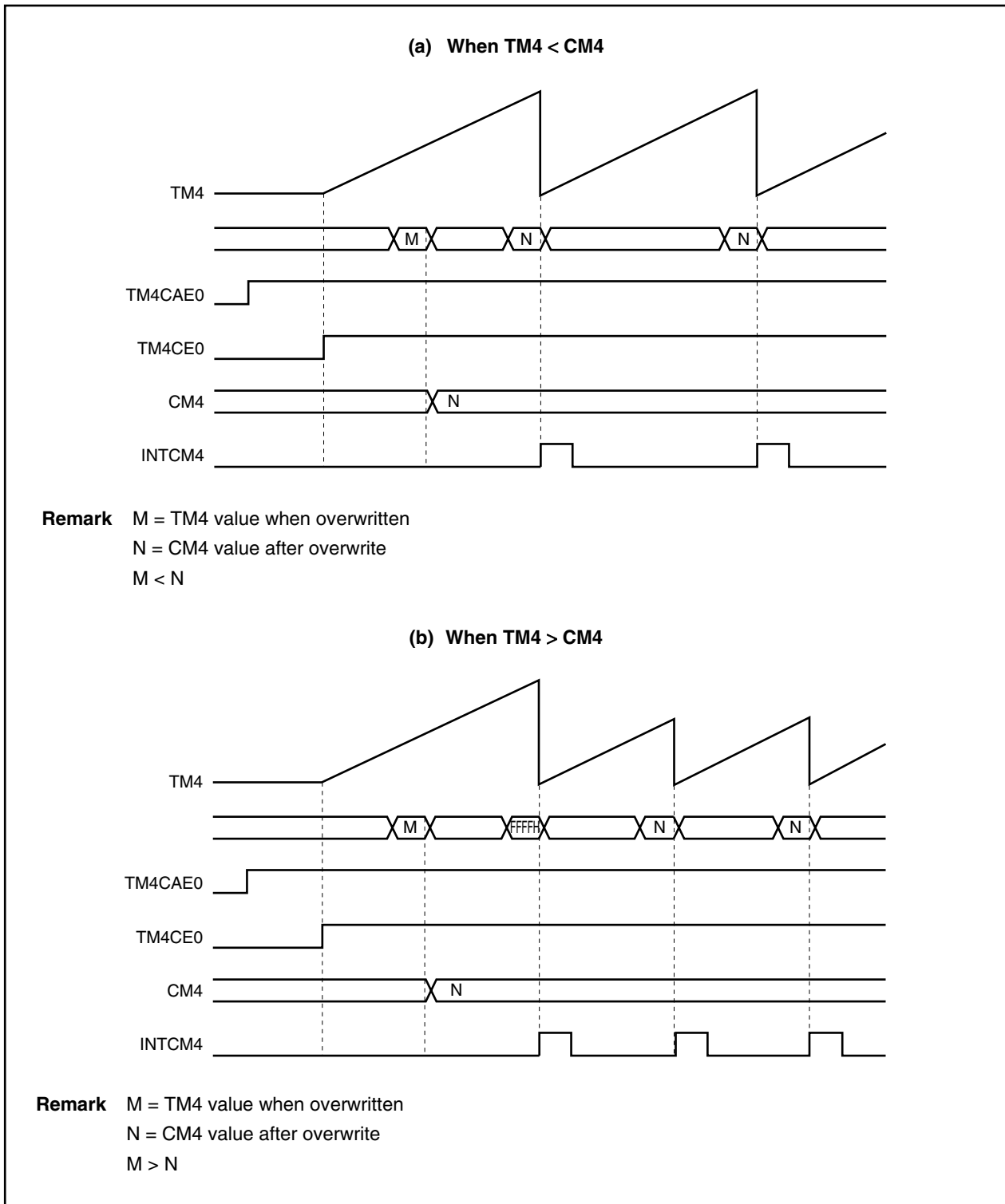
Figure 9-104. Example of Timing During TM4 Operation
