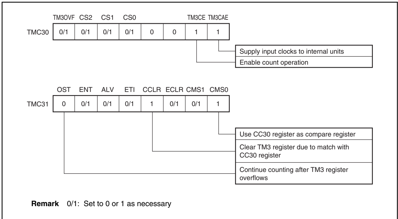
Figure 9-97. Contents of Register Settings When Timer 3 Is Used as Interval Timer
