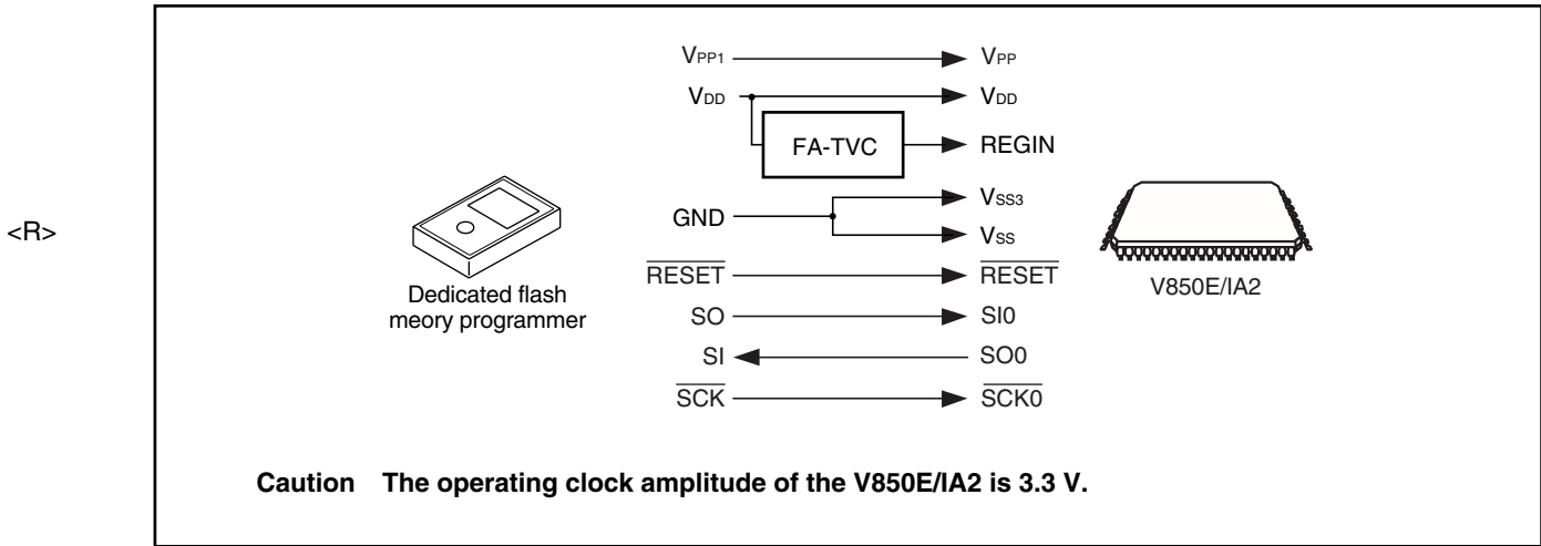
Figure 15-3. Communication with Dedicated Flash Memory Programmer (CSIO)
