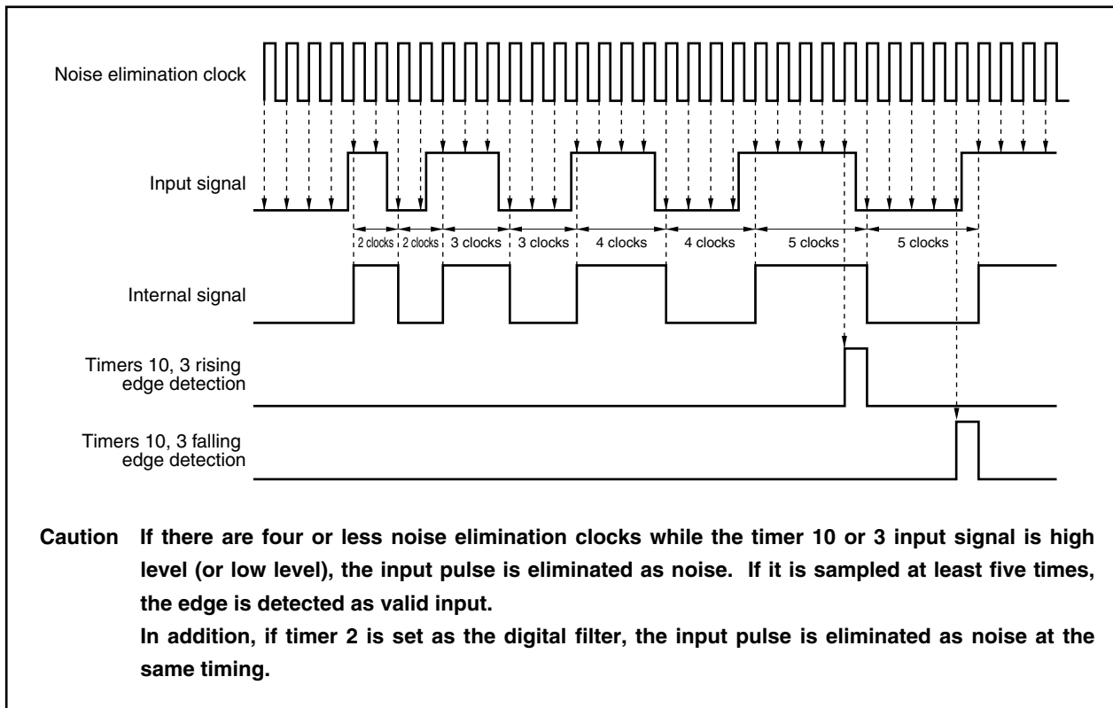
Figure 12-15. Example of Noise Elimination Timing
