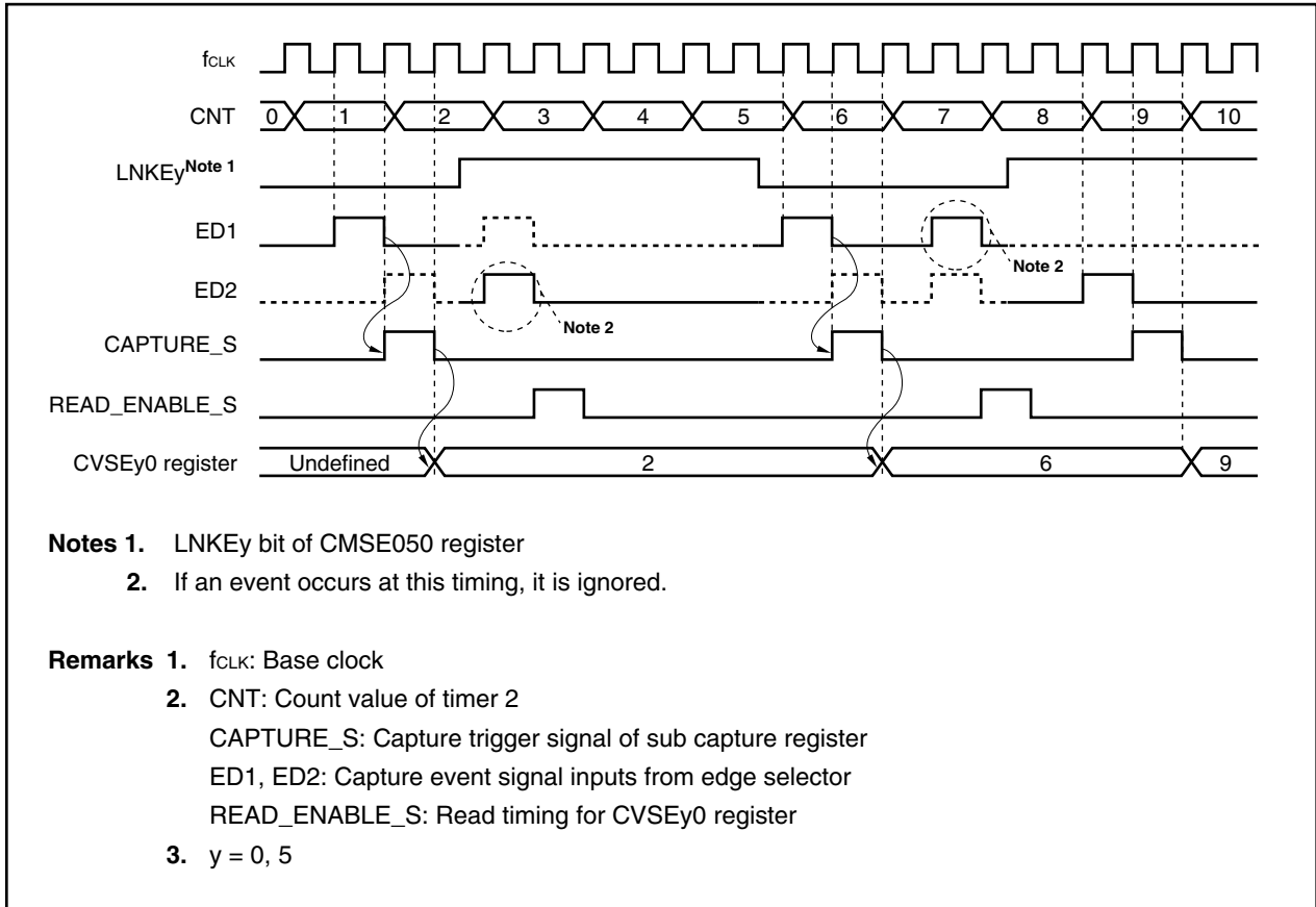
Figure 9-80. Capture Operation: Timer 2 Count Value Read Timing (When CMSE050 Register's CCSEy Bit = 0, EEVEy Bit = 1, and CSCE0 Register's SEVEy Bit = 0)
