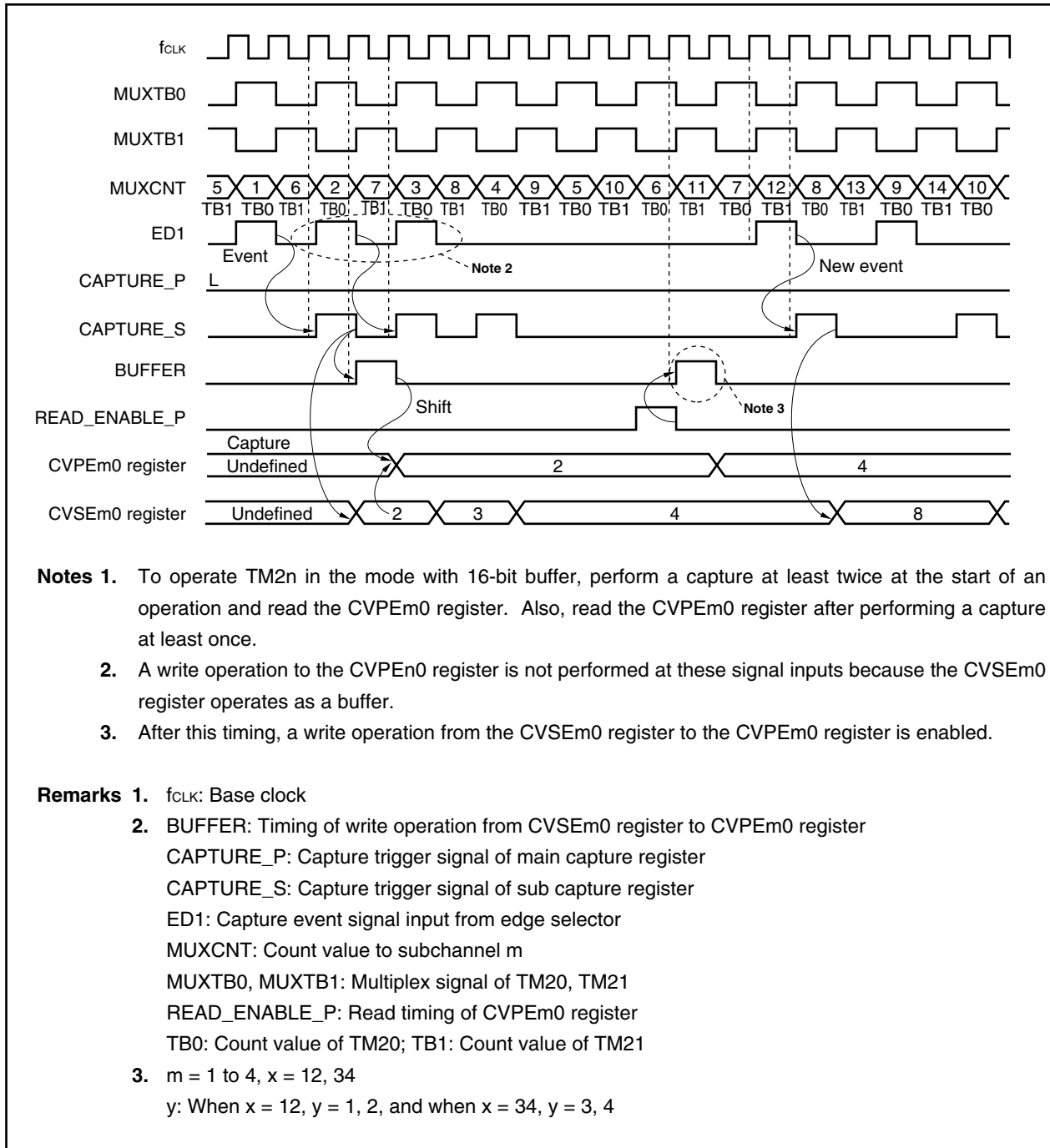
Figure 9-75. Capture Operation: Mode with 16-Bit Buffer Note 1 (When CMSEx0 Register's TByE1 Bit = 0, TByE0 Bit = 1, CCSEy Bit = 0, LNKEy Bit = 0, BFEEy Bit = 1, EEVEy Bit = 1, and CSCE0 Register's SEVEy Bit = 0)
