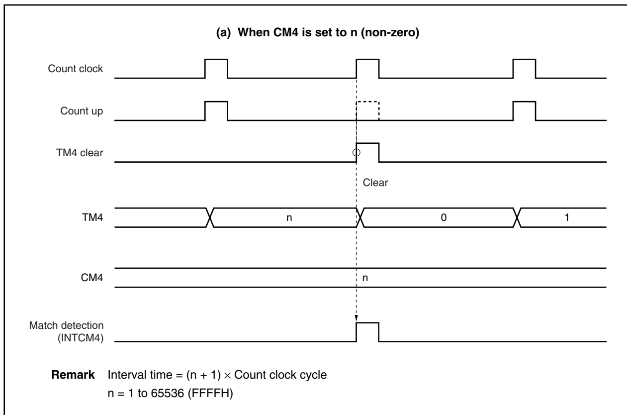
Figure 9-105. TM4 Compare Operation Example (1/2)
