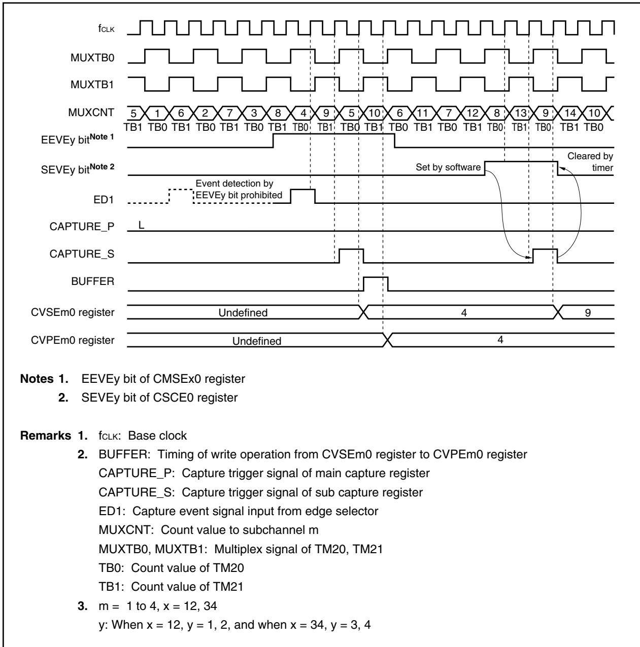
Figure 9-77. Capture Operation: Capture Control by Software and Trigger Timing (When CMSEx0 Register's TByE1 Bit = 0, TByE0 Bit = 1, CCSEy Bit = 0, LNKEy Bit = 0, BFEEy Bit = 1)
