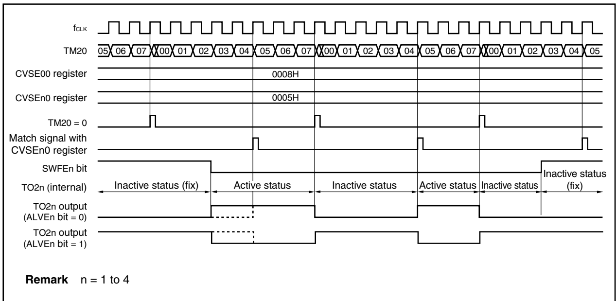
Figure 9-87. When Normal Output Operation Starts/Ends
