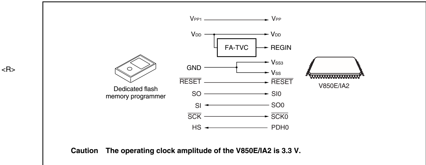
Figure 15-4. Communication with Dedicated Flash Memory Programmer (Handshake-Supported CSI Communication)
