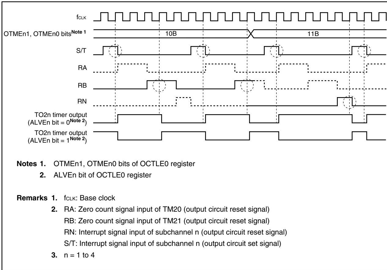
Figure 9-84. Signal Output Operation: During Software Control (When OCTLE0 Register's OTMEn1, OTMEn0 Bits = Arbitrary, SWFEn Bit = 1, and ODELE0 Register's ODLEn2 to ODLEn0 Bits = 0)
