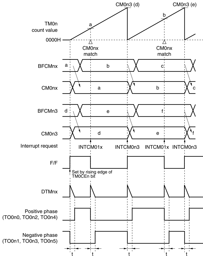
(a) Operation timing of compare registers 0n0 to 0n2 (CM0n0 to CM0n2)
