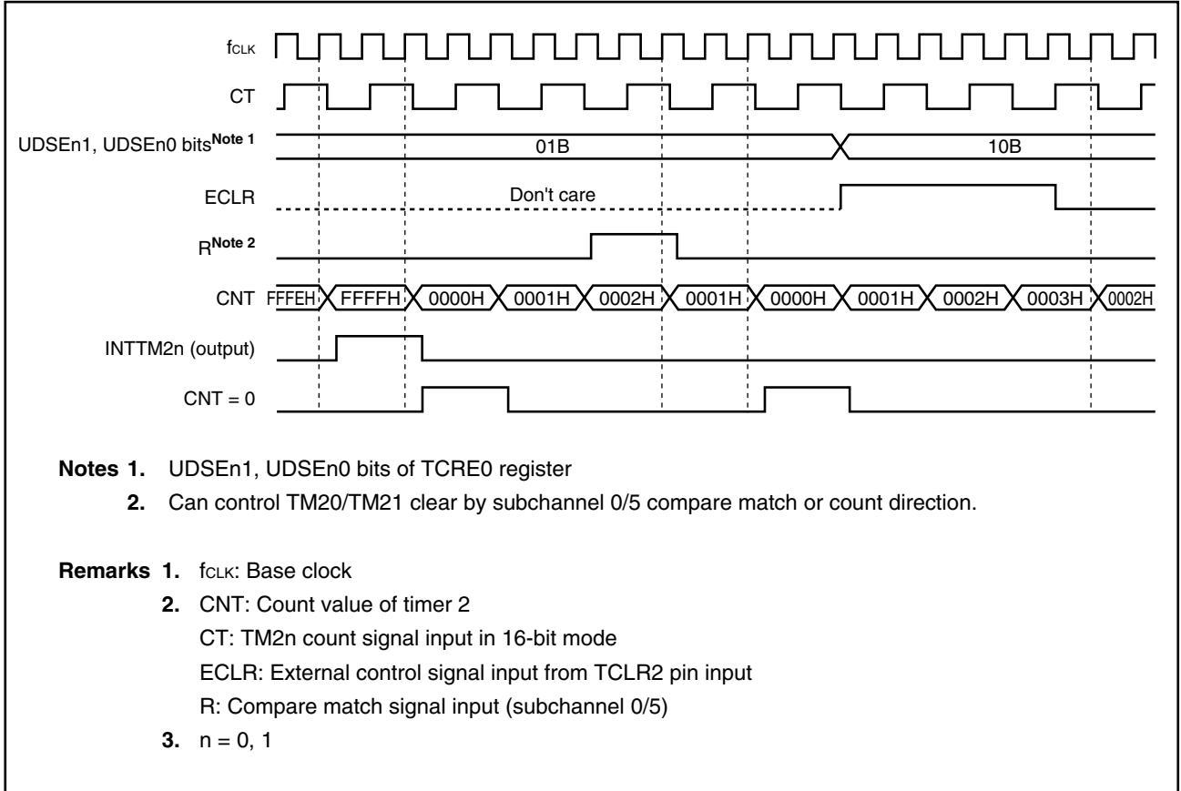
Figure 9-70. Operation in Timer 2 Count Up/Down Mode (When TCRE0 Register's ECEEn bit = 0, ECREn Bit = 0, CLREn Bit = 0, OSTEn Bit = 0, CEEn Bit = 1, CASE1 Bit = 0)
