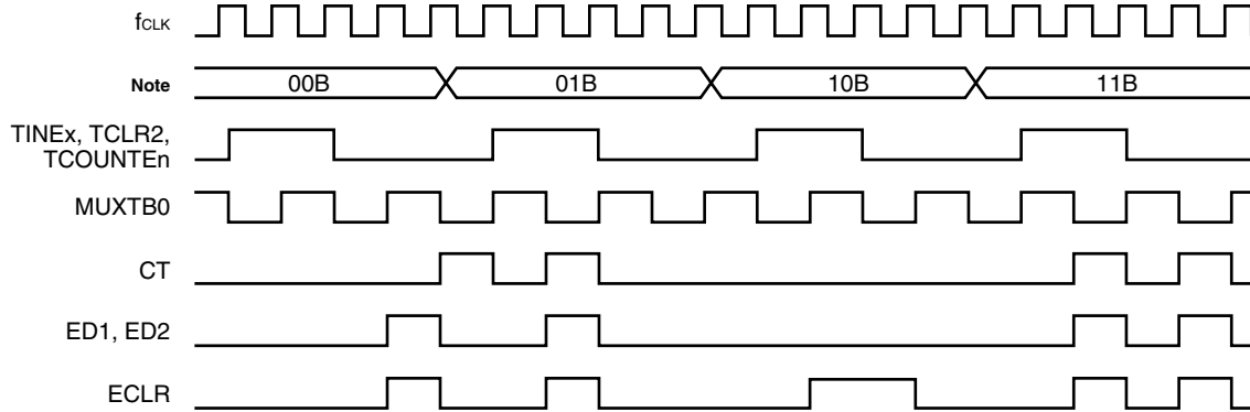
Figure 9-67. Edge Detection Timing
