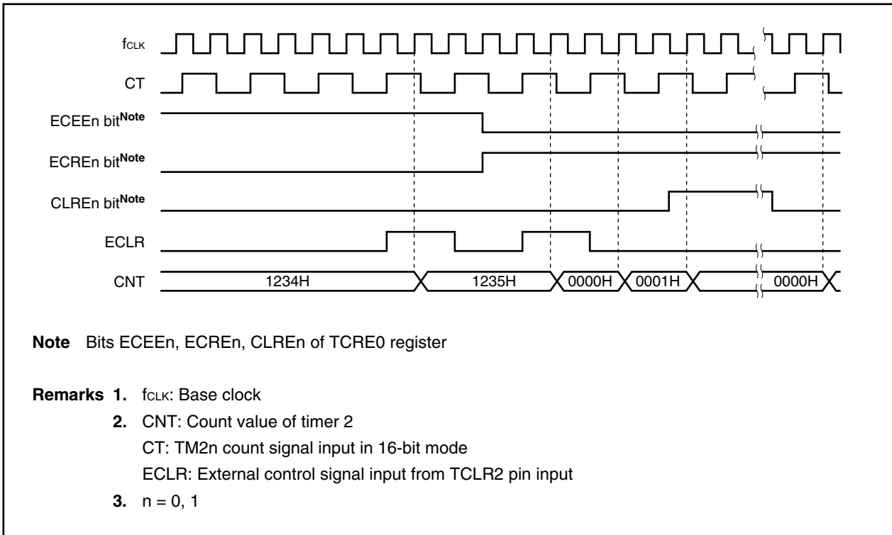
Figure 9-69. External Control Timing of Timer 2 (When TCRE0 Register's UDSEn1, UDSEn0 Bits = 00B, OSTEn Bit = 0, CEEEn Bit = 1, CASE1 Bit = 0)
