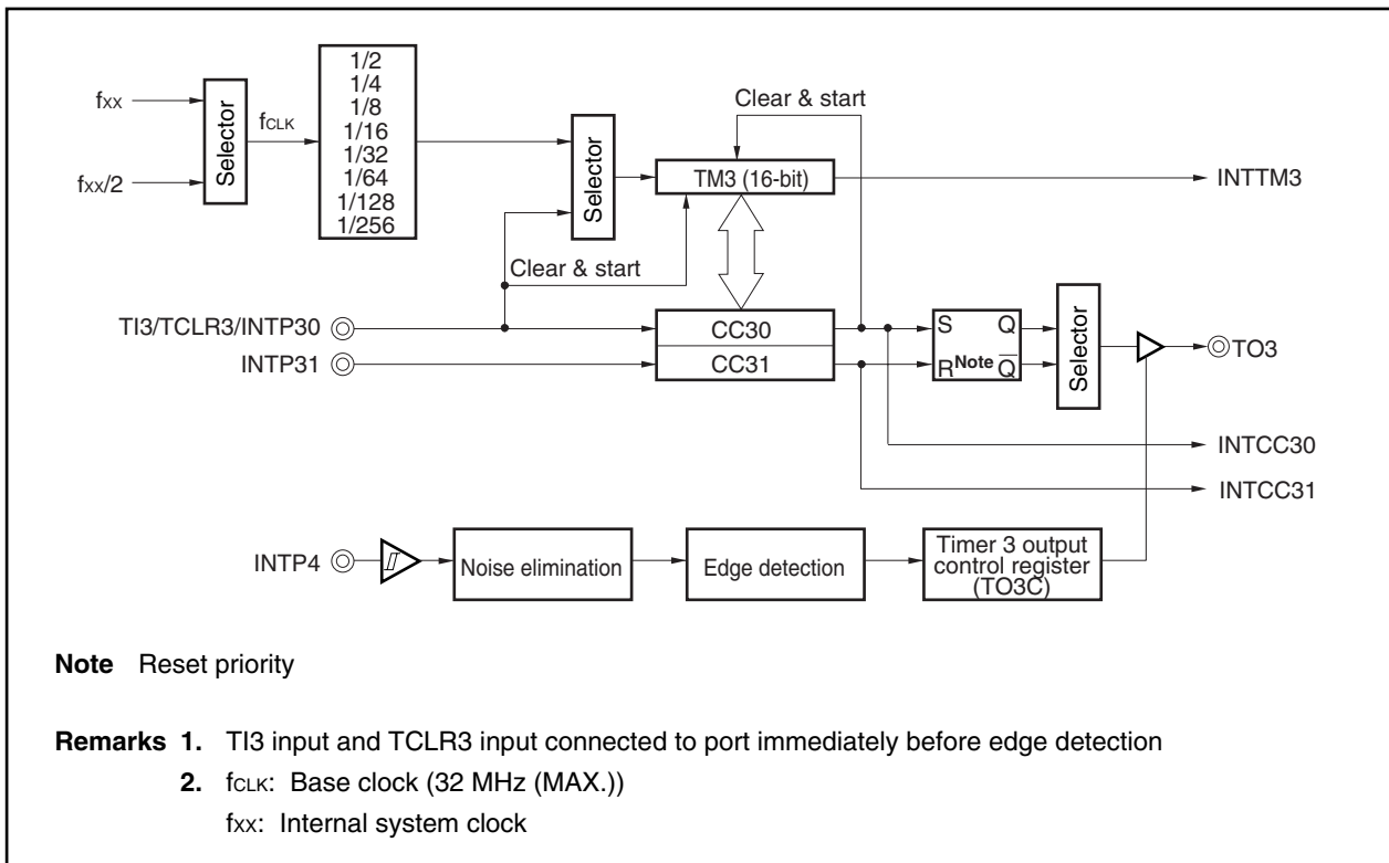
Figure 9-89. Block Diagram of Timer 3
