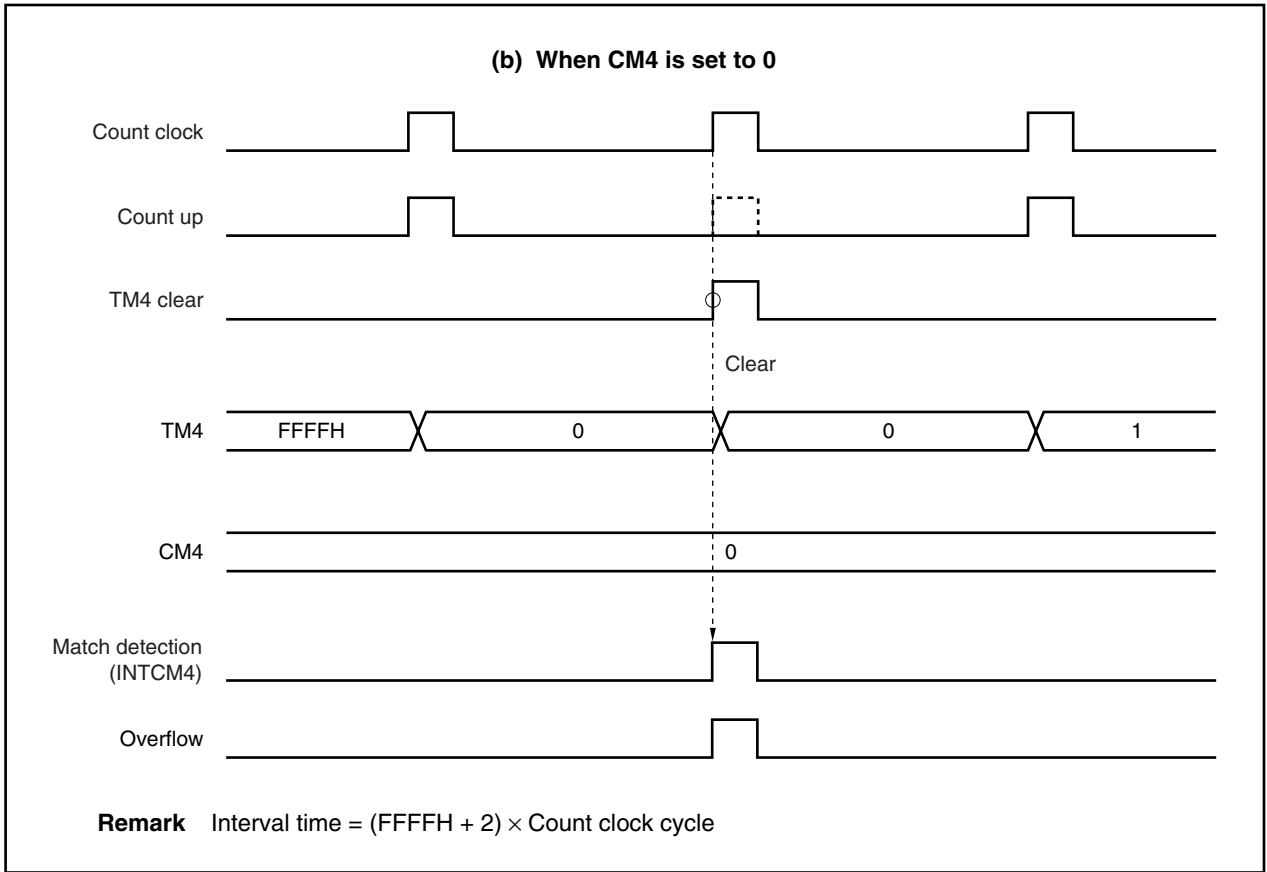
Figure 9-105. TM4 Compare Operation Example (2/2)
