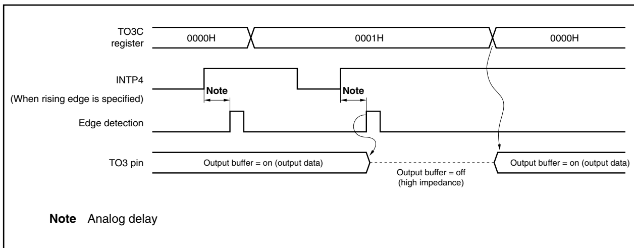
Figure 9-96. Example of Operation of TO3 Output Control Function by INTP4 Pin (in TO3 Output Mode (PMC27 Bit = 1 and PFC27 Bit = 1))
