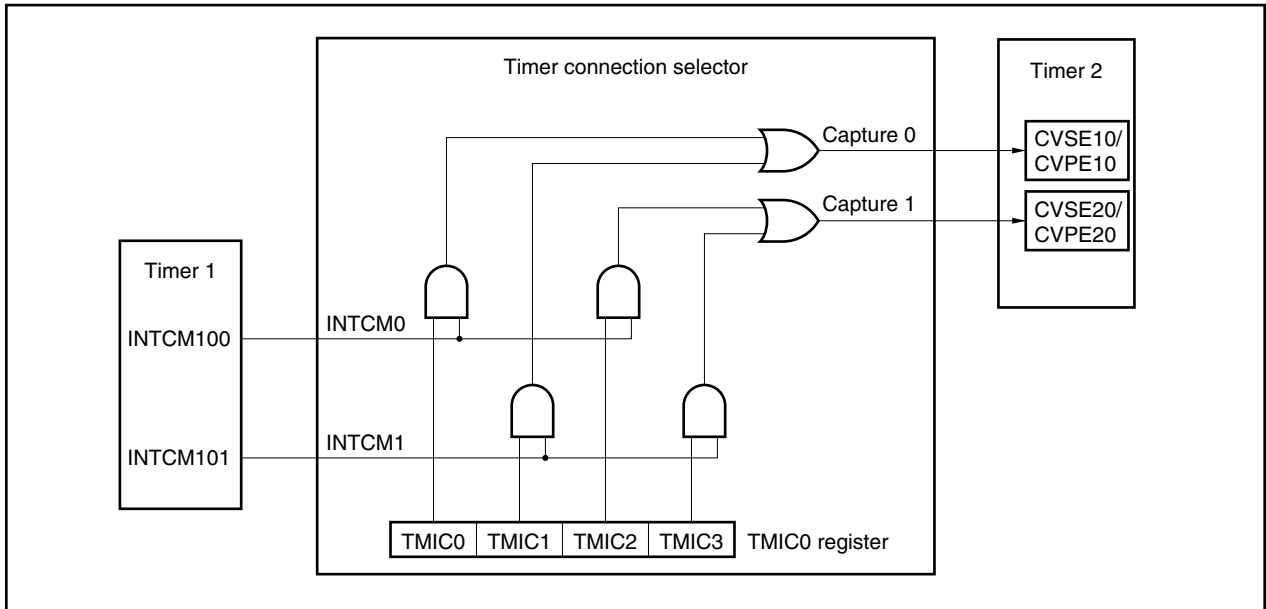
Figure 9-106. Block Diagram of Timer Connection Function
