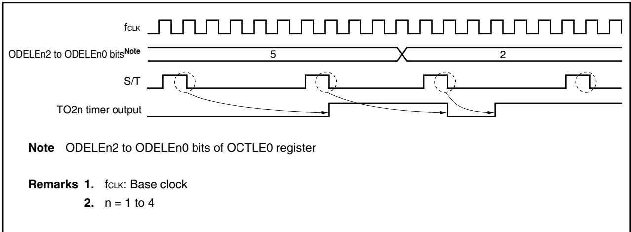
Figure 9-85. Signal Output Operation: During Delay Output Operation (When OCTLE0 Register's OTMEn1, OTMEn0 Bits = 0, ALVEn = 0, SWFEn Bit = 0)
