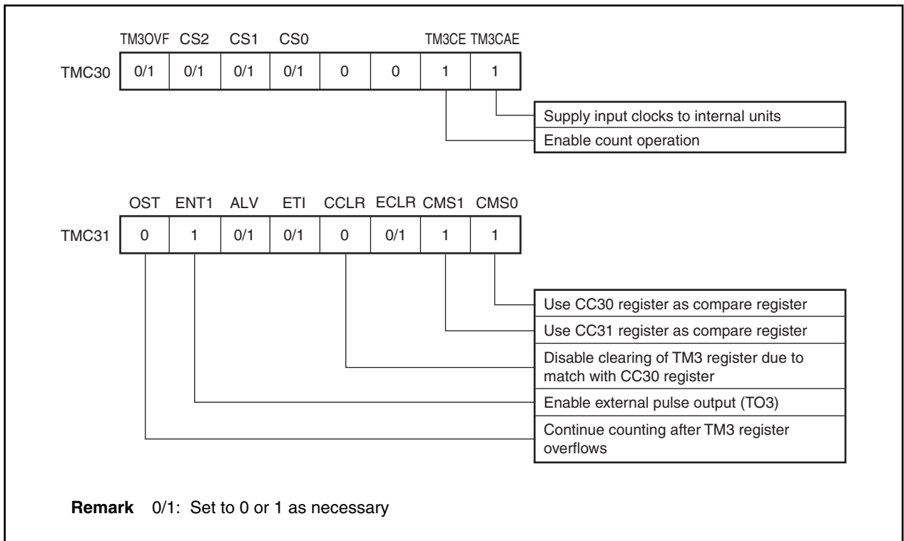
Figure 9-99. Contents of Register Settings When Timer 3 Is Used for PWM Output
