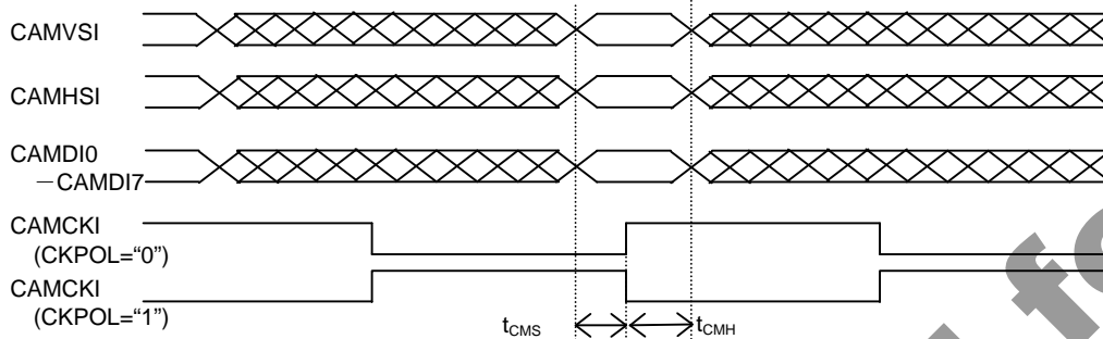
Fig.5 Data Input Interface Timing
