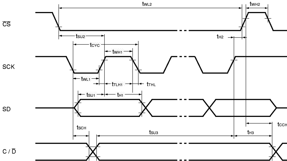
Fig. 2 Interface timing
