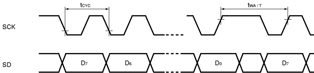
Fig. 3 Command cycle
