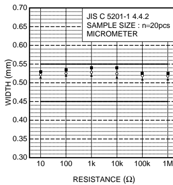
Fig.3 Dimensions (width)
