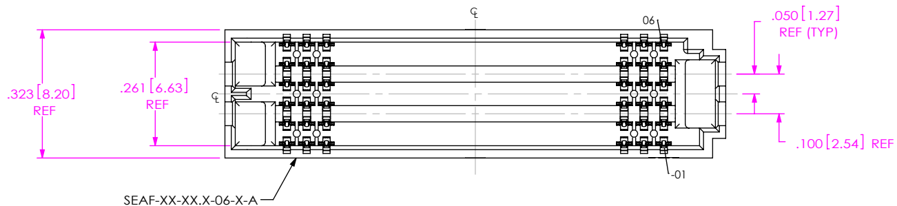
FIG 4 -06: 6 ROW (SAME AS FIG 1, EXCEPT AS SHOWN) (SEAF-20-05.0-XX-06-1-A-XX-K-TR SHOWN) (SOME CENTER FEATURES REMOVED FOR CLARITY)
