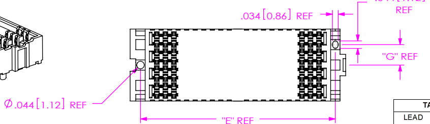
FIG 1 -08: 8 ROW (SEAF-20-05.0-XX-08-1-A-XX-K-TR SHOWN) (SOME CENTER FEATURES REMOVED FOR CLARITY)
