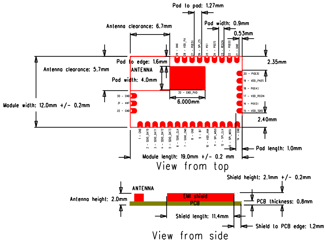
Figure 11: Physical dimensions
