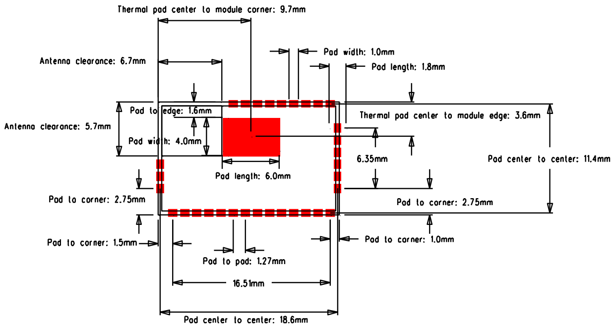
Figure 12: WF111 recommended PCB land pattern
