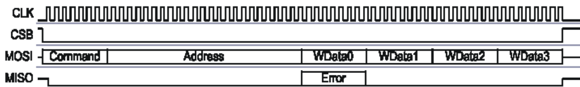
Figure 5: CSPI Burst Write Cycle
