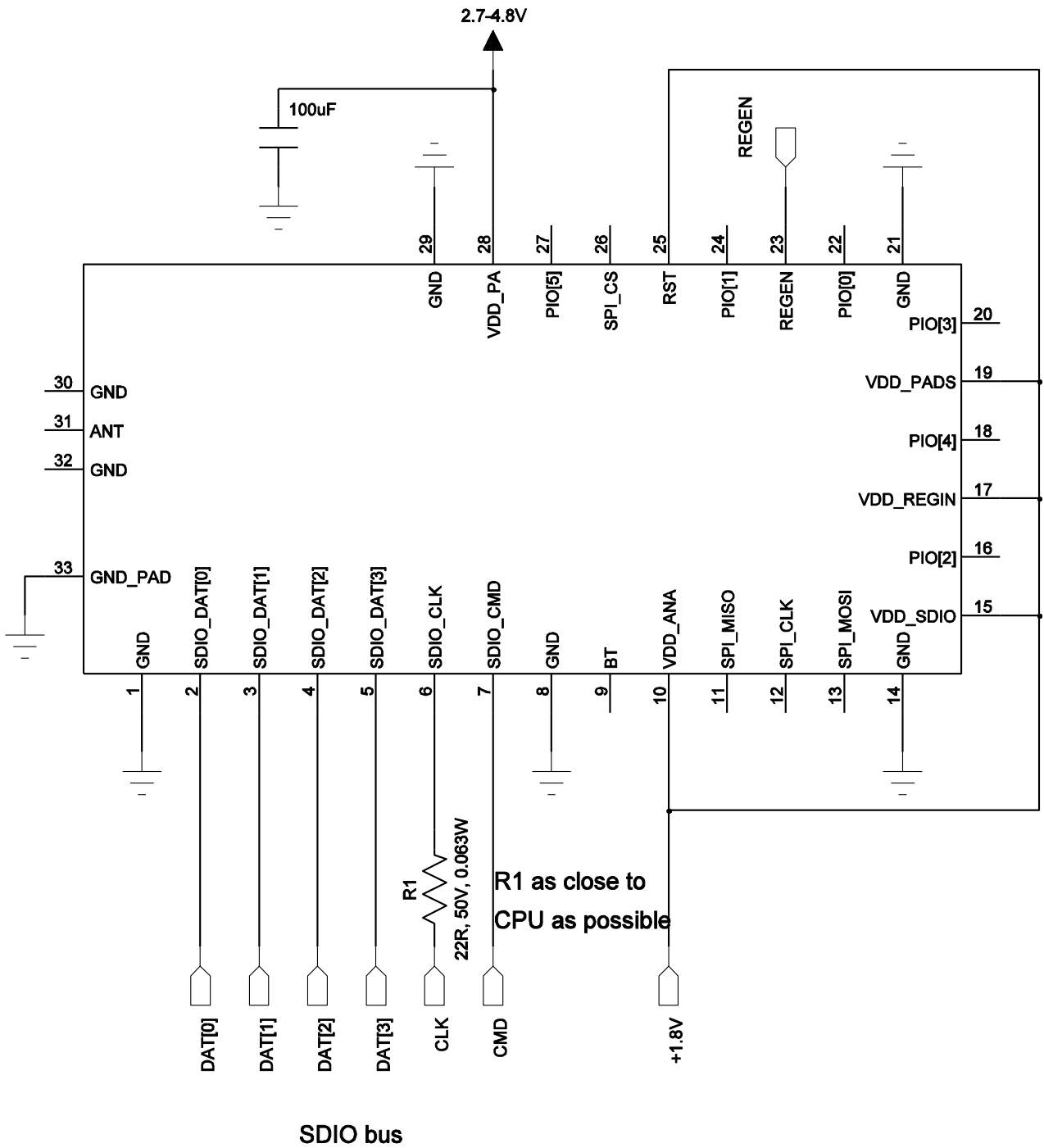
Figure 10: An example application circuit with SDIO host connection, 1.8V level host logic and a separate power amplifier supply, RST hard wired to the core supply and REGEN pad used to power off and reset the module (Note: with N-variant ANT-pad and associated grounds would also be connected)
