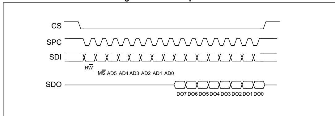
Figure 5. SPI read protocol
