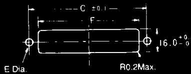
Panel Cutout
