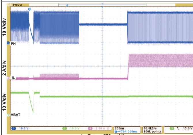
Figure 9. Battery Insertion
