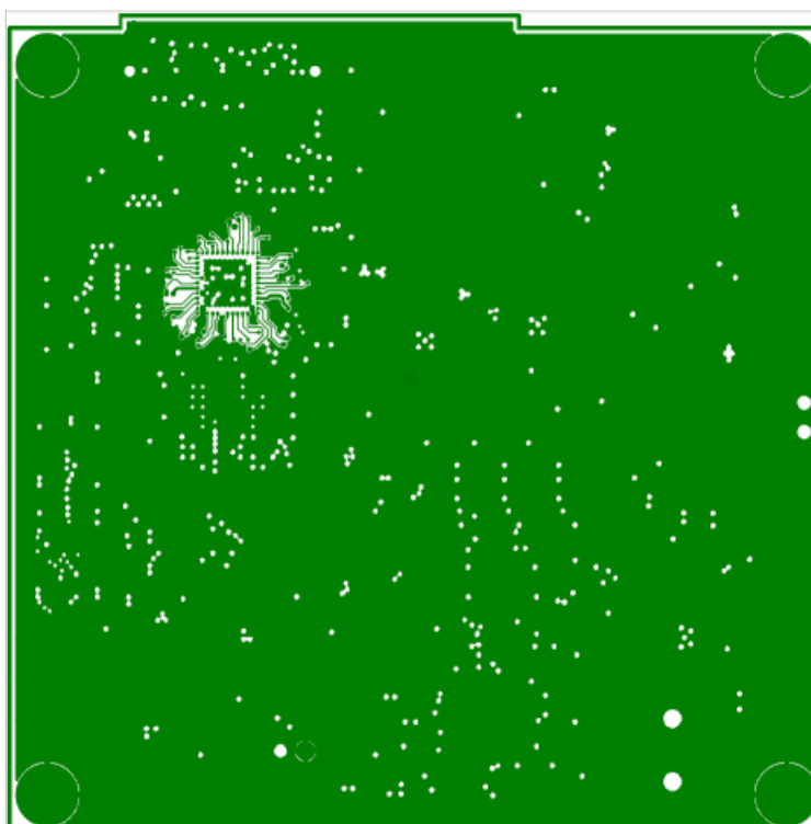
Figure 22. Internal Layer
