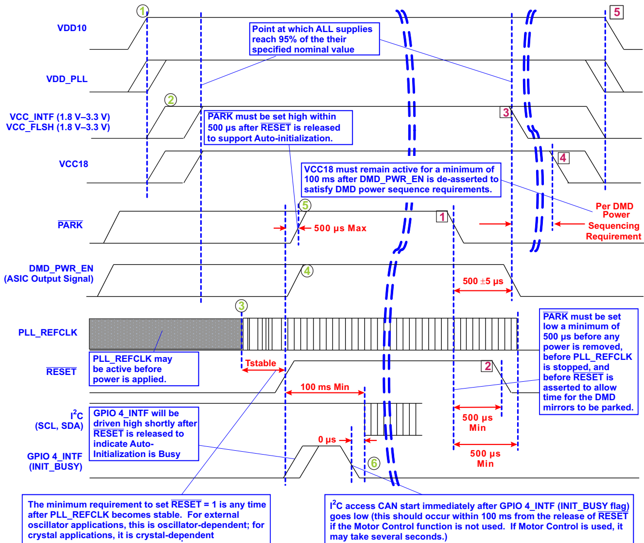
Figure 17. Power-Up/Down Timing
