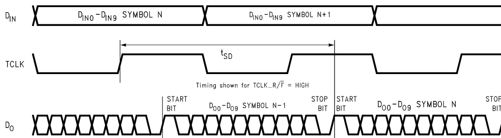
Figure 9. Serializer Delay
