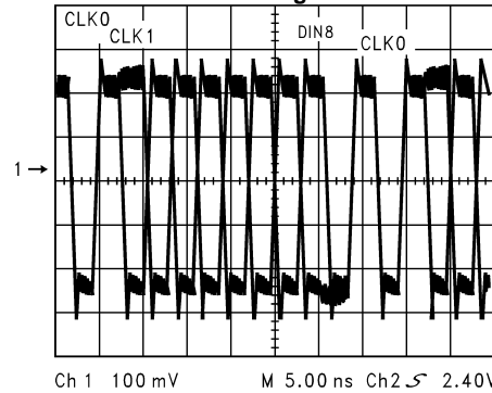
Figure 1. RMT Patterns Seen on the Bus LVDS Serial Output
