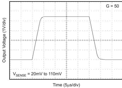
Figure 14. Step Response
