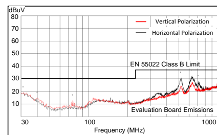
Radiated Emission Graph V_{OUT} = 3.3 V, V_{IN} = 24 V, F_S = 500 kHz, I_{OUT} = 1 A
