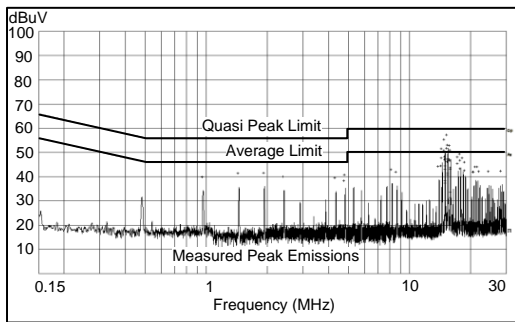
V_{OUT} = 3.3\text{ V} F_S = 500\text{ kHz} I_{OUT} = 1\text{ A} Measured on the LM46001QPWPEVM with default BOM. EVM input filter: L_{in} = 1\text{ }\mu\text{H} C_d = 47\text{ }\mu\text{F} C_{IN4} = 68\text{ }\mu\text{F}
