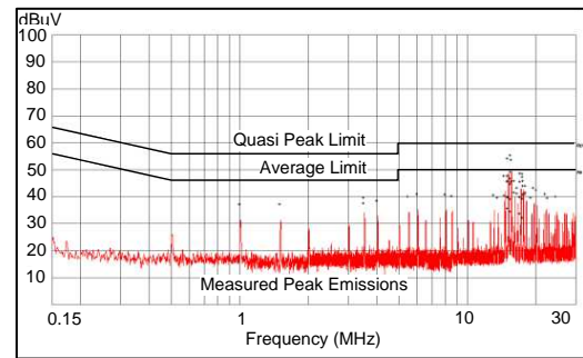
V_{OUT} = 5\text{ V} F_S = 500\text{ kHz} I_{OUT} = 1\text{ A} Measured on the LM46001QPWPEVM with L = 27\text{ }\mu\text{H} , C_{OUT} = 66\text{ }\mu\text{F} , C_{FF} = 33\text{ pF} . EVM input filter L_{in} = 1\text{ }\mu\text{H} C_d = 47\text{ }\mu\text{F} C_{IN4} = 68\text{ }\mu\text{F}
