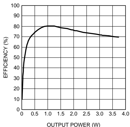
Figure 9. Boost Amplifier vs Output Power V_{DD} = 5\text{ V}, R_L = 8\ \Omega f = 1\text{ kHz}, PV_1 = 7.8\text{ V}
