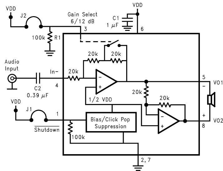
Figure 26. REFERENCE DESIGN BOARD SCHEMATIC
